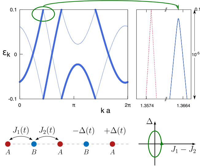
FIG. 1. Top left: quasienergy spectrum of the Rice-Mele model \Delta_0 = 3J_0 , \delta_0 = J_0 , \omega = 0.2J_0/\hbar . The thick band is the lowest-energy Floquet band \varepsilon_{LE,k} . Top right: (solid line) enlargement of the previous figure close to the upper border of the FBZ around ka = 1.3664 ; the dashed line denotes the quasienergies in the adiabatic limit \varepsilon_{\alpha,k}^0 . Notice the gap of order 10^{-6} . Bottom: A cartoon of the Rice-Mele model (left) and a path in parameter space.
