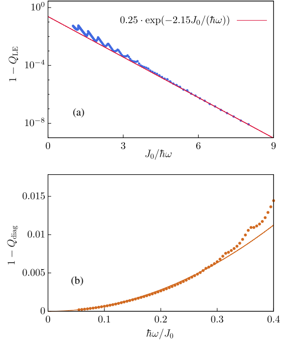
FIG. 2. (a) The deviation from 1 of the charge pumped by the lowest-energy Floquet band (proportional to the sum of gaps) as a function of 1/\hbar\omega , with its exponential fit (red solid straight line). (b) Deviations from 1 of the diagonal pumped charge Q_{\text{diag}} in the RM model for a sudden switch on of the driving. The smooth curve \frac{9}{128}(\hbar\omega/J_0)^2 is obtained from Eq. (6). The model parameters are \Delta_0 = 3J_0 , \delta_0 = J_0 .
