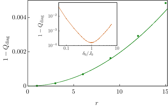
FIG. 3. Deviations from the integer value of the diagonal pumped charge Q_{\text{diag}} in the RM model versus the aspect ratio r = \Delta_0/\delta_0 of the driving ellipse for \delta_0 = J_0 , for a sudden switch on of the driving with frequency \omega = 0.05J_0/\hbar . The smooth curve is \frac{1}{128}(\hbar\omega/J_0)^2 r^2 and it was calculated with the first order perturbative calculation of the main text. In the inset, the deviation from 1 of Q_{\text{diag}} for a fixed r = 3 as a function of \delta_0 : The minimum sits at \delta_0 = J_0 .
