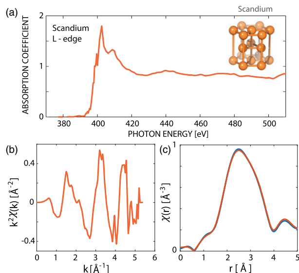
FIG. 3. Experimental XAFS spectroscopy near the Sc L edge, using a 2\ \mu\text{m} -driven HHG supercontinuum up to 550 eV. (a) The normalized absorption coefficient of Sc near the L -absorption edge at 398 eV. (b) k^2 -scaled EXAFS function in k space extending to >5\ \text{\AA}^{-1} . (c) Experimental R -space EXAFS function (blue), not corrected for \delta phase shifts, and fitted (red) to theory. The real-space EXAFS function exhibits a broad peak. Inset shows a Sc hcp unit cell.
