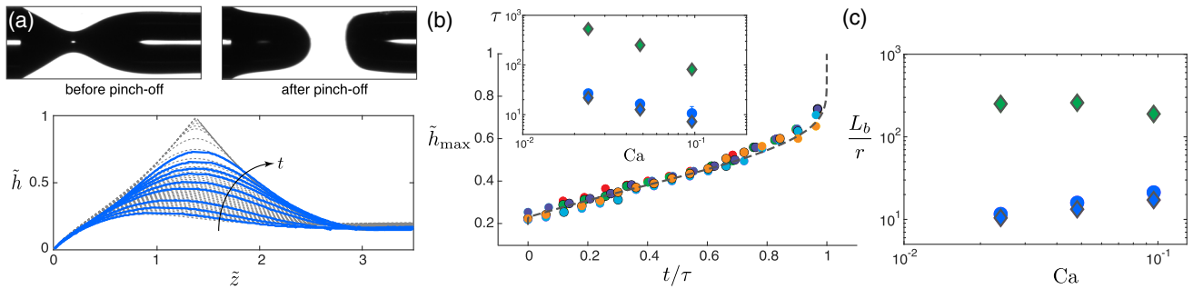
FIG. 4. (a) Top: experimental images of the fluid-fluid interface profile just before and after pinch-off. Bottom: the dewetting rim profile in the frame comoving with the receding contact line for \text{Ca} = 0.096 and \theta_{\text{eq}} = 68^\circ . The dashed and solid lines correspond to the numerical and experimental data, respectively. (b) The maximum height of the rim \tilde{h}_{\text{max}} grows linearly at early times and nonlinearly accelerates close to the pinch-off time \tau . The color-coded circles represent different experimental realizations of rim growth that led to pinch-off, while the dashed line represents the theoretical prediction of Eq. (2). The inset shows the pinch-off time as a function of the capillary number and the wettability condition, where the green and blue symbols correspond to \theta_{\text{eq}} = 25^\circ and 68^\circ , respectively. The theoretical predictions (diamonds) match closely to the experimental data (circles) for \theta_{\text{eq}} = 68^\circ . Given the limited experimental window, we did not directly observe pinch-off in the more wetting tube since its \tau is predicted to be over an order of magnitude larger than that in the less wetting tube. (c) The bubble length L_b as a function of the capillary number and the wettability condition, where the green and blue symbols correspond to \theta_{\text{eq}} = 25^\circ and 68^\circ , respectively. The theoretical predictions (diamonds) agree well with the experimental data (circles) for \theta_{\text{eq}} = 68^\circ . See the video [22].
