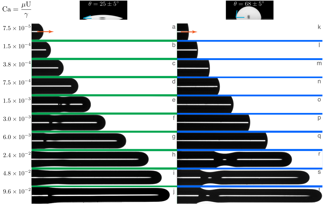
FIG. 1. Fluid-fluid interface of air (black) displacing glycerol (white) under increasing capillary numbers (top to bottom) in a wetting capillary tube with \theta_{\text{eq}} = 25^\circ \pm 5^\circ (left column) and a weakly wetting capillary tube with \theta_{\text{eq}} = 68^\circ \pm 5^\circ (right column). The orange arrows indicate the direction of interface displacement. At small Ca , the meniscus deforms slightly from its equilibrium shape, but remains as a spherical cap. At large Ca , however, a wetting transition occurs and the invading air forms a single finger that advances along the center of the tube, leaving a macroscopic trailing film of the viscous liquid on the tube walls. The critical capillary number Ca^* at which film formation occurs is controlled by the wettability [pane (r) versus pane (e)].
