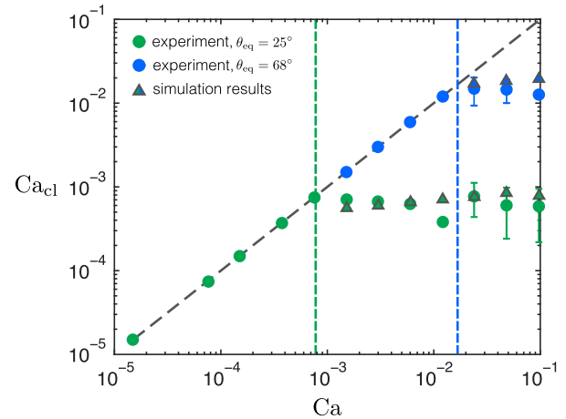
FIG. 3. The contact line capillary number Ca_{cl} = \mu U_{cl}/\gamma as a function of the macroscopic capillary number Ca = \mu U/\gamma , where U_{cl} and U are the contact line velocity and the displacement velocity, respectively. The green and blue circles represent the experimental measurements in the more wetting tube ( \theta_{eq} = 25^\circ ) and in the less wetting tube ( \theta_{eq} = 68^\circ ), respectively. The triangles show the corresponding theoretical predictions of Eq. (2). The vertical dashed lines represent the critical capillary numbers Ca^* as predicted by Eq. (1). For Ca < Ca^* , the fluid-fluid interface deforms slightly while remaining a spherical cap, and the contact line and the interface tip travel at the imposed displacement velocity U = 4Q/\pi d^2 (gray dashed line). For Ca > Ca^* , the air forms a finger that advances along the center of the tube, leaving behind a film of the more-viscous defending liquid. The incomplete displacement of the defending liquid results in an interface tip velocity that is larger than the imposed displacement velocity. The contact line that trails behind travels at a velocity that, remarkably, is independent of the imposed flow rate. Instead, the contact line velocity is controlled by the wettability of the capillary tube.
