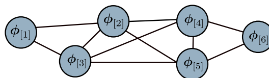
FIG. 1. A network of quantum sensors. The k th node represents a sensor into which the vector parameter \phi_{[k]} is encoded via a local unitary evolution. The connections between the nodes denote that, in general, the sensors can be entangled, and/or global measurements can be performed.
