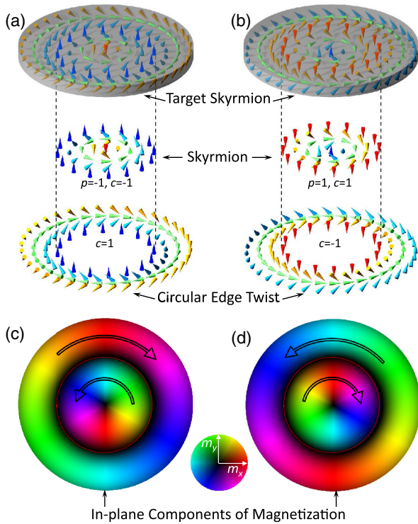
FIG. 1. (a) and (b) Magnetization configurations of twofold-degenerate target Skyrmions for p = -1 and p = +1 , respectively. (c) and (d) In-plane magnetization in the target Skyrmions in (a) and (b), respectively, with colors and arrows used to indicate the rotational sense of the in-plane magnetization, according to the color wheel shown. The dashed black lines in (a) and (b) and the thin red lines in (c) and (d) mark the boundaries between the Skyrmions and the circular edge twists.
