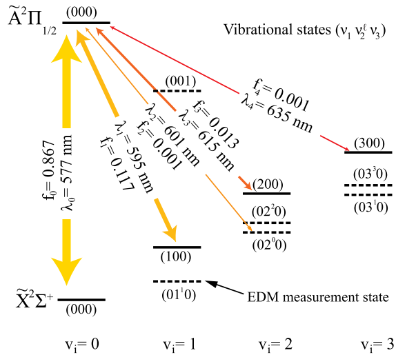
FIG. 3. Proposed photon cycling and laser-cooling scheme for YbOH. Thicker lines indicate stronger transitions with appropriate Franck-Condon factors ( f ) and wavelengths ( \lambda ) indicated. The energy splittings are not to scale.
