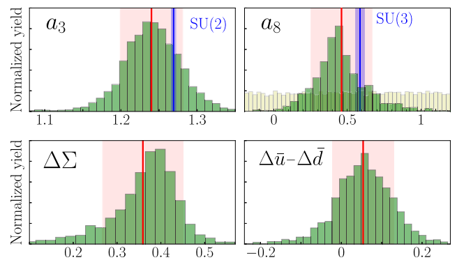
FIG. 4. Normalized yield of the lowest moments of the spin-dependent PDFs for the triplet ( a_3 ), octet ( a_8 ), and singlet ( \Delta\Sigma ) axial charges, and the flavor asymmetry \Delta\bar{u} - \Delta\bar{d} , with average values (red vertical lines) and 1\sigma deviations (pink bands) indicated at the input scale. For the scale invariant a_3 [ a_8 ], the SU(2) [SU(3)] symmetric values are indicated (blue vertical bands), together with the flat prior distributions for a_8 without SU(3) (yellow histograms).
