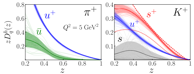
FIG. 3. Fragmentation functions z D_q^h(z) to \pi^+ (left panel) and K^+ (right panel) for u^+ (blue), \bar{u} (green), s^+ (red), and s (grey) at Q^2 = 5 \text{ GeV}^2 for the JAM17 analysis. Random samples of 50 posteriors are shown with the mean and variance, and compared with the s^+ \rightarrow K^+ FFs from DSS [62] (dashed curve) and HKNS [63] (dotted curve).
