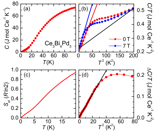
FIG. 5. (a) Temperature-dependent specific heat C(T) of \text{Ce}_3\text{Bi}_4\text{Pd}_3 below 100 K. (b) C/T vs T^2 below 14 K, in zero field and 7 T. The slope \beta of the black straight line corresponds to the phonon contribution C_{\text{ph}} ; the red and blue (steepest) lines with steeper slope \beta' are interpreted as Weyl contributions (see the text). (c) Entropy of electronic specific heat C_{\text{el}} = C - C_{\text{ph}} vs temperature. (d) With the lowest- T CDW and NFL contributions (see Fig. S3 in the Supplemental Material [20]) subtracted, linear-in- T^2 behavior (the black line) of C_{\text{el}}/T prevails from 0.4 to 5.5 K.
