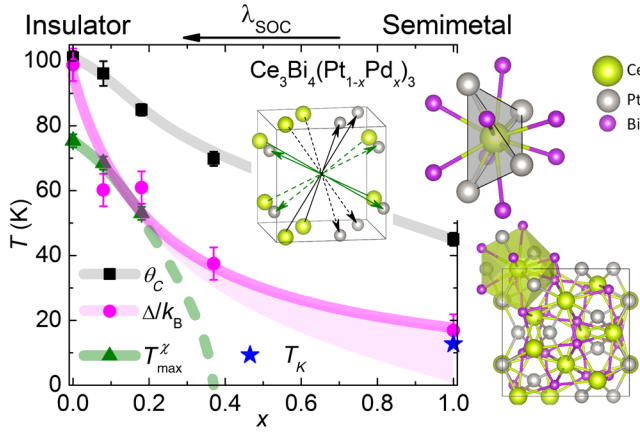
FIG. 3. Characteristic temperature scales for \text{Ce}_3\text{Bi}_4(\text{Pt}_{1-x}\text{Pd}_x)_3 as a function of x . T_{\text{max}}^{\chi} and \Theta_C are taken from Fig. 4(a) and the Curie-Weiss fits in Fig. 4(b), respectively. \Delta/k_B is taken from the Arrhenius fits in Figs. 2(b) and 2(c). The Kondo temperature T_K is taken from the entropy analysis in Fig. 5(c). The full lines are guides for the eye. The shaded pink (light gray) area represents the fact that, for x = 1 , the Arrhenius fit loses significance and R(T) becomes compatible with a gapless state (see the text). The dashed green line indicates that the maximum in \chi(T) is suppressed to below 2 K for x = 0.37 . The arrow on the top axis indicates that an increase of the conduction-electron \lambda_{\text{SOC}} (corresponding to a decrease of x ) drives the system from a semimetallic to an insulating state. The structure sketches illustrate the unit cell (bottom), the environment of Ce with the four nearest Pt/Pd (3.01 Å) and eight next-nearest Bi (3.41 Å) neighbors (top), and the lack of a center of inversion for (selected) Ce and Pt atoms (left).
