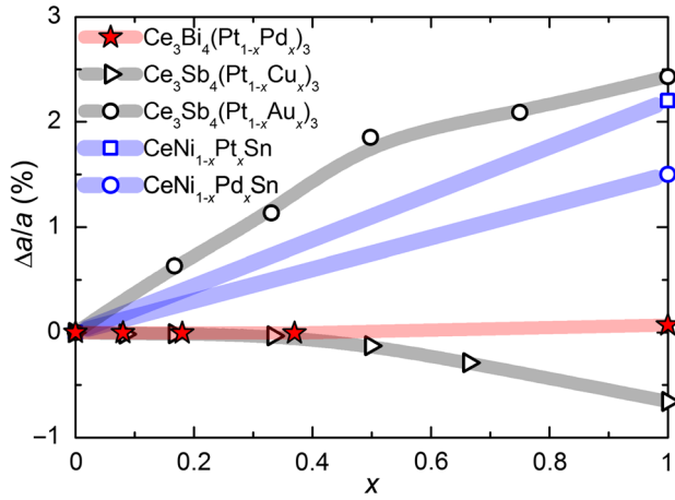
FIG. 1. Relative change of lattice parameter a as function of the Pd content x in \text{Ce}_3\text{Bi}_4(\text{Pt}_{1-x}\text{Pd}_x)_3 (red, stars), on a scale relevant to other archetypal Kondo systems [31–34] (the open symbols). The lines are guides for the eye.
