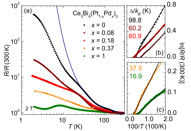
FIG. 2. (a) Temperature-dependent electrical resistance R(T) , normalized to its room temperature value R(300\text{K}) , on a log-log scale for all investigated \text{Ce}_3\text{Bi}_4(\text{Pt}_{1-x}\text{Pd}_x)_3 samples. Labels reflect order of the curves at low temperatures. An exponentially activated resistivity, fitted to the high-temperature regime of the x = 0 sample, is shown as a blue line. (b),(c) Arrhenius plots for data above 50 K. The solid lines are the fits (see the text). The data for the x = 1 sample were taken at 2 T to suppress a spurious superconducting resistance drop at 3 K that has no correspondence in magnetization and specific heat measurements. This magnetic field has no effect on the resistance data above 3 K.
