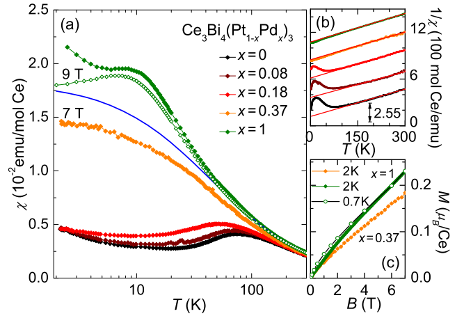
FIG. 4. (a) Temperature-dependent magnetic susceptibility \chi(T) of all investigated \text{Ce}_3\text{Bi}_4(\text{Pt}_{1-x}\text{Pd}_x)_3 samples, together with the Curie-Weiss fit for the x = 1 data [the blue line, from (b)]. Labels reflect inverse order of the data sets at low temperatures. (b) \chi^{-1} vs T along with the Curie-Weiss fits that determine the paramagnetic Weiss temperature \Theta_C . The data for x > 0 are successively shifted by 255 molCe Oe/emf for clarity. Unless specified, the field for the data in (a) and (b) was 100 mT. (c) Selected magnetization vs field M(B) isotherms. The slight nonlinearities at low fields indicate that the low-temperature upturn of \chi(T) , seen most clearly for the x = 1 sample in (a), is readily saturable by small fields.
