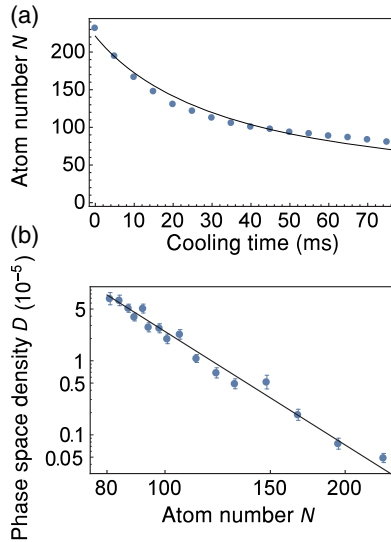
FIG. 3. (a) Atom number extracted from the total scattering rate into the cavity. The solid line is a two-body loss model fitted to the experimental data with a fitted two-body loss coefficient of 0.12(1) 1/s . (b) Phase space density D as a function of the remaining atom number. A linear fit between \ln(D) and \ln(N) is plotted as a solid line. The fit gives \gamma = 5.0(3) .
