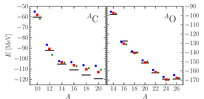
FIG. 2. Ground-state energies for even carbon and oxygen isotopes obtained from the IM-NCSM at N_{\max} = 4 (square) in comparison to importance-truncated NCSM calculations with explicit 3N interactions (circle) and the multireference IM-SRG with HF-Bogoliubov reference states (triangle) [32]. Experimental values are indicated by black bars [46]. The uncertainty due to flow-parameter dependence is negligible on this scale.
