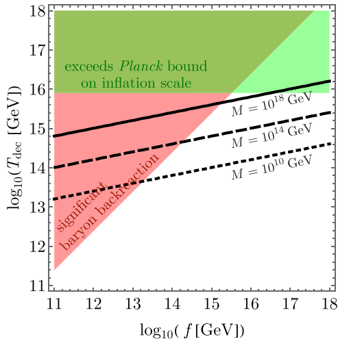
FIG. 1. Parameter space in the f - T_{\text{dec}} plane. The colored regions are excluded due to a significant backreaction from the baryons (red area) and by the Planck upper bound on the inflation scale (green area). The allowed parameter space is shown in white. The black lines indicate where the right amount of baryon asymmetry is produced, for the choice of M = 10^{18} (solid line), 10^{14} (dashed line), and 10^{10} GeV (dotted line).
