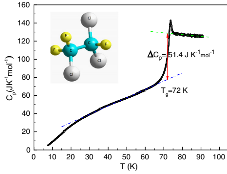
FIG. 1. Specific heat of Freon 113 [35] around the glasslike transition, T_g = 72 K.
