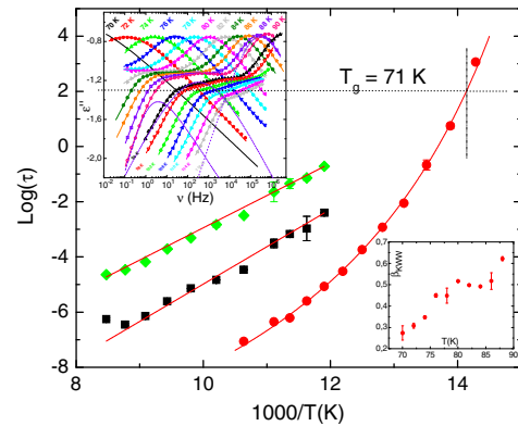
FIG. 3. Relaxation time as a function of reciprocal temperature for both \alpha (red circles) and slower (green diamonds and black squares) relaxations. Top left inset shows obtained dielectric spectra for several temperatures ranging from 70 to 90 K. Solid lines are examples of the fits using Havriliak-Negami and Cole-Cole functions (dashed lines for the spectrum at 88 K) for the main \alpha relaxation and the slower processes, respectively. Bottom right inset collects the \beta^{\text{KWW}} exponent as a function of temperature.
