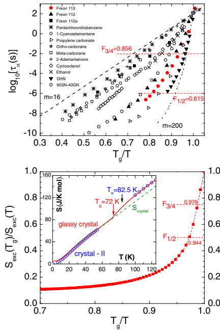
FIG. 4. (Top panel) \tau_\alpha as a function of T_g/T (Angell plot). VFT parameters for Freon 113 are T_0=58.9\pm 0.6 K, \tau_0=(2.9\pm 1.6)\times 10^{-12} s, D=(6.4\pm 0.5) . Fragility index is m=127 . (Bottom panel) Reciprocal of the excess entropy—normalized by the excess entropy at T_g —as a function of T_g/T . Inset: Entropy for the plastic and glassy crystal phases (red solid line), for the stable crystal II and the liquid (blue points, from Ref. [38]) as a function of temperature. The green dashed line indicates the extrapolation of the crystal II as a reference for higher temperatures. In both (top panel) and (bottom panel), the dashed lines drawn at the 1/2 and 3/4 marks are used to obtain either kinetic (top panel) or thermodynamic (bottom panel) fragilities F_{1/2} and F_{3/4} , respectively.
