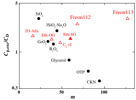
FIG. 5. Excess heat capacity C_{p,\text{exc}} = C_p - C_D , at the boson-peak maximum in C_p/T^3 scaled to C_D , as a function of the fragility index m in a semilogarithmic scale. Black circles correspond to canonical glasses, taken from the original figure from Ref. [37]. We have added some data (red triangles) from this (Freon 113) and earlier works: adamantanone (2O-Ada) [39], cyclohexanol ( \text{C}_6\text{-ol} ) [40], Freon 112 [31], and ethanol both as orientational (Eth-OG) and structural (Eth-SG) glass [41,42]. Solid symbols indicate structural glasses and open symbols indicate orientational glasses.
