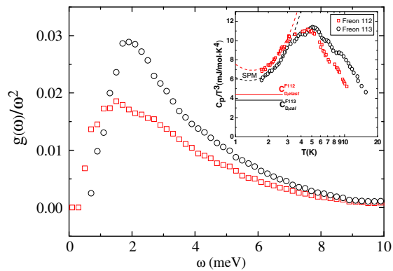
FIG. 2. Debye-reduced vibrational density of states divided by \omega^2 for Freon 112 (red squares) and for Freon 113 (black circles) determined at 5 K by means of inelastic neutron scattering at the MARI spectrometer. Inset: Molar heat capacity divided by T^3 for Freon 112 and Freon 113 [35], the calculated Debye values, and the fits (dashed lines) corresponding to the soft potential model in a semilogarithmic plot.
