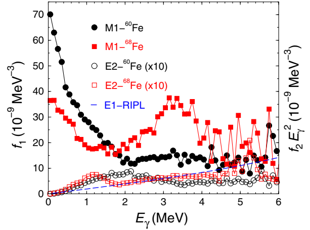
FIG. 4. Strength functions deduced from the present calculations for ^{60}\text{Fe} and ^{68}\text{Fe} . Dipole strength functions f_1 deduced from average B(M1) values are shown as filled black circles for ^{60}\text{Fe} and filled red squares for ^{68}\text{Fe} . The E1 strength function according to the RIPL data base [5] is shown as a blue dashed line. Quadrupole strength functions f_2 deduced from average B(E2) values and multiplied with the transition energies are shown as open black circles and open red squares for ^{60}\text{Fe} and ^{68}\text{Fe} , respectively. Note that the f_2 E_\gamma^2 were multiplied by a factor of 10 to make them better visible.
