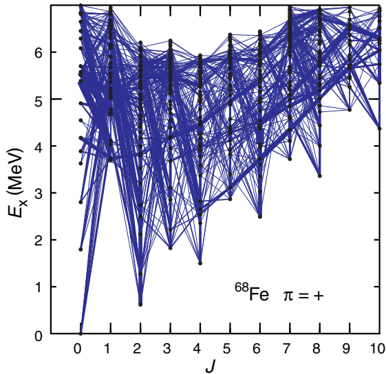
FIG. 3. Transitions with B(M1) > 0.1\mu_N^2 (blue lines) between the calculated positive-parity states (black dots) in ^{68}\text{Fe} . The widths of the lines are proportional to the B(M1) values.
