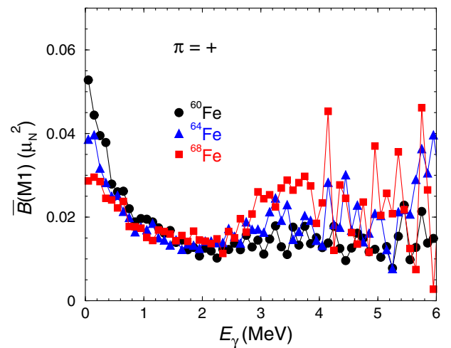
FIG. 1. Average B(M1) values in 100 keV bins of transition energy calculated for positive-parity states in ^{60}\text{Fe} (black circles), ^{64}\text{Fe} (blue triangles up), and ^{68}\text{Fe} (red squares).
