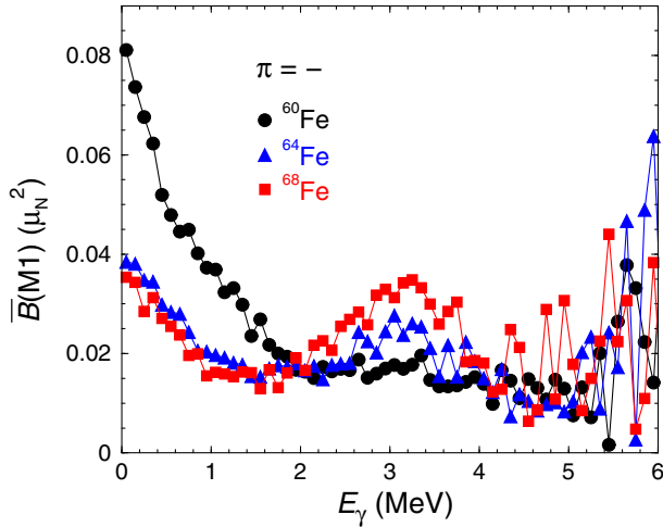
FIG. 2. As Fig. 1, but for negative-parity states.
