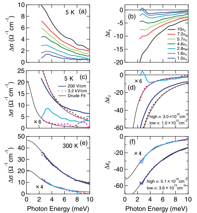
FIG. 2. (a),(b) Pair density dependence of (a) \Delta\sigma(\omega) and (b) \Delta\epsilon(\omega) spectra obtained with the weak THz probes at t_{pp} = 10 ps, from 1.0n_0 to 10n_0 with n_0 = 1.0 \times 10^{15} \text{ cm}^{-3} . (c),(d) Comparison of the weak and the strong THz probe spectra of (c) \Delta\sigma(\omega) and (d) \Delta\epsilon(\omega) at T_{\text{lattice}} = 5\text{ K} , at the low density 1.0 \times 10^{15} \text{ cm}^{-3} and the high density 3.0 \times 10^{16} \text{ cm}^{-3} . The spectra taken by weak (strong) THz probe pulses are shown as solid (dashed) lines, and thin black solid lines are the fitted result of strong THz probe spectra with the Drude model. (e),(f) Comparison of the weak and the strong THz probe spectra of (e) \Delta\sigma(\omega) and (f) \Delta\epsilon(\omega) at t_{pp} = 10 ps and at T_{\text{lattice}} = 300\text{ K} .
