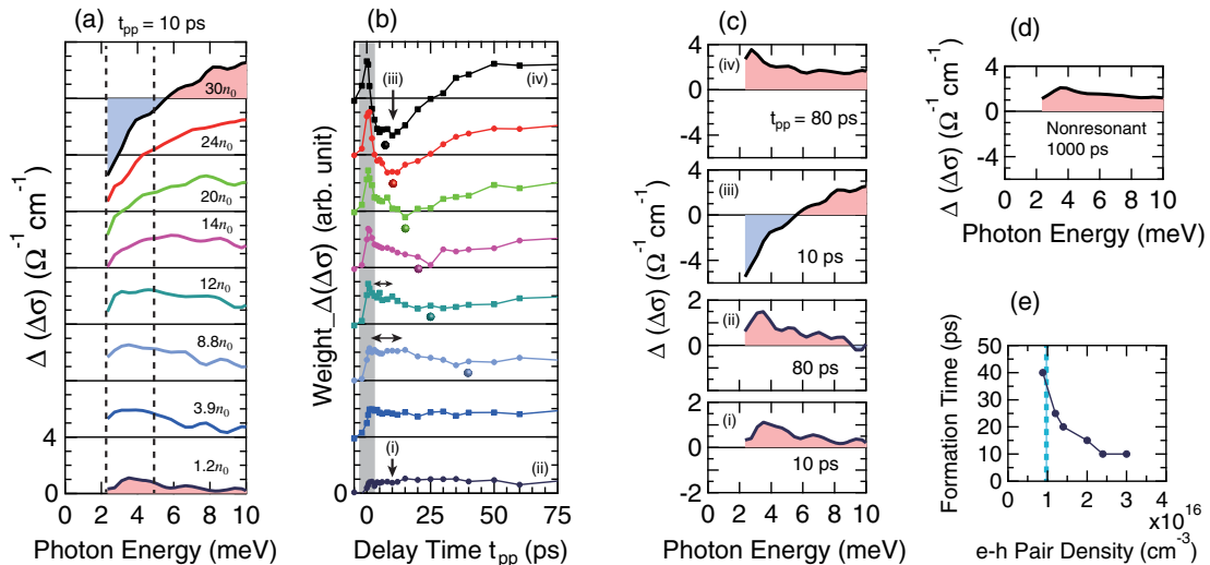
FIG. 4. (a) Differential optical conductivity spectra \Delta(\Delta\sigma(\omega)) at t_{pp} = 10 ps at different densities. (b) Spectral weight dynamics of the \Delta(\Delta\sigma(\omega)) integrated in the region between the dashed lines in (a). The gray-shaded area indicates the region where the pump and probe pulses temporally overlap. (c) \Delta(\Delta\sigma(\omega)) spectra at the lowest (i and ii) and the highest (iii and iv) density, at t_{pp} = 10 ps (i and iii) and 80 ps (ii and iv), indicated in (b). (d) \Delta(\Delta\sigma(\omega)) spectrum under the condition of nonresonant excitation ( \sim 8 meV above the band edge) at high density 2.7 \times 10^{16} \text{ cm}^{-3} and at t_{pp} = 1000 ps, which corresponds to the quasithermal equilibrium condition at T \sim 5 K. (e) The density dependence of the formation time of the CM. Dashed line indicates n_{\text{Mott}} .
