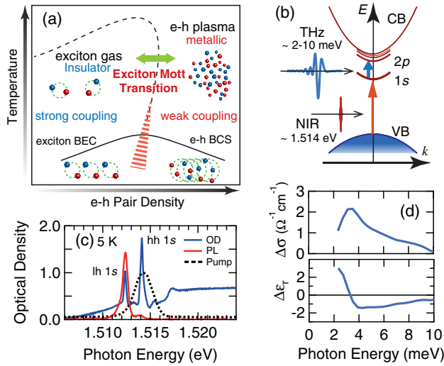
FIG. 1. (a) Schematic phase diagram of e - h systems in photoexcited semiconductors. (b) Energy diagram of our OPTP measurement. (c) Solid blue line: near-infrared optical density spectrum of the sample around the band edge. Solid red line: photoluminescence spectrum under the above-gap excitation condition. Dashed line: spectrum of the optical pump. (d) Photo-induced changes of the real part of (top panel) optical conductivity \Delta\sigma(\omega) and (bottom panel) dielectric function \Delta\epsilon(\omega) .
