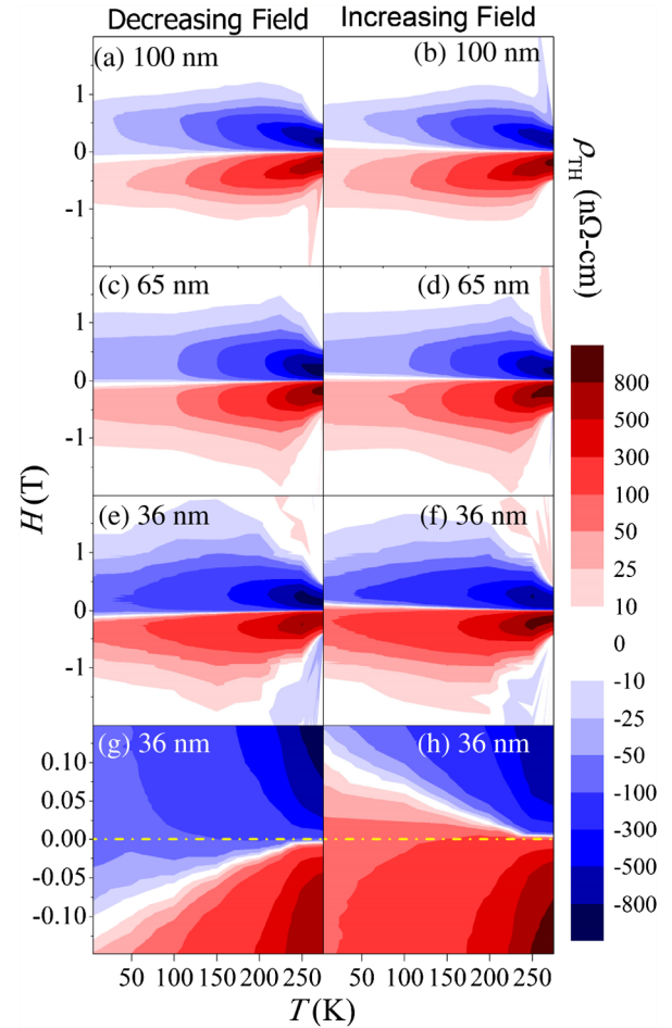
FIG. 4. Contour plots of \rho_{\text{TH}} for the (a),(b) 100 nm, (c),(d) 65 nm, and (e)–(h) 36 nm FeGe films. The plots on the left have the field sweeping from +7 to –7 T, and the plots on the right have the field sweeping in the opposite direction. A zoom-in view of the 36 nm film in (g) and (h) highlights that nonzero topological Hall resistivity exists at a zero field for all temperatures, particularly at low temperatures with substantial remanence at H = 0 .
