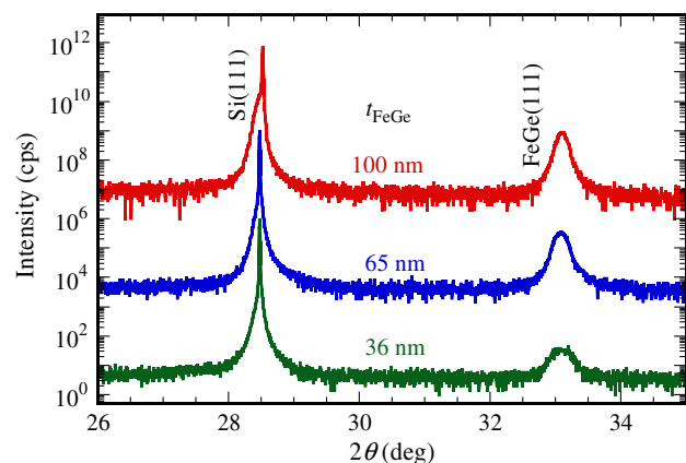
FIG. 1. Semilog 2\theta - \omega XRD scans of 100, 65, and 36 nm FeGe films epitaxially grown on Si(111).
