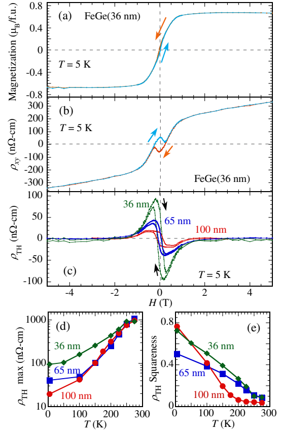
FIG. 3. (a) Out-of-plane magnetic hysteresis loop of the 36 nm FeGe film at 5 K. (b) Total Hall resistivity ( \rho_{xy} ) of the 36 nm FeGe film with a coercivity of 2400 Oe ( T = 5 K) reveals a dominant topological Hall effect, which has a path opposite of the expected anomalous Hall effect. (c) The topological Hall resistivity ( \rho_{TH} ) hysteresis loops for the 36, 65, and 100 nm FeGe films at 5 K show a clear Skyrmion phase, which exhibit substantial remanent values at H = 0 , demonstrating robust Skyrmion formation in the absence of magnetic field. (d) Semilog plot of the temperature dependence of the maximum \rho_{TH} for the three samples. (e) The squareness of the topological Hall resistivity \rho_{TH}(H = 0)/\rho_{TH}(\max) for the three FeGe films between 5 and 275 K, reflecting the stability of Skyrmions at zero field.
