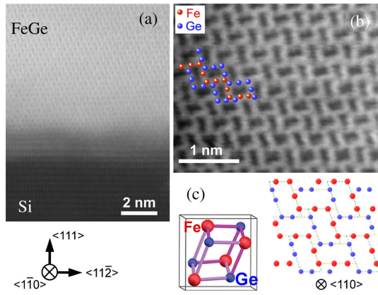
FIG. 2. (a) STEM image of a 100 nm FeGe thin film viewed along the FeGe \langle 110 \rangle axis near the interface with Si(111). A 1.2–1.5 nm interfacial transition region is observed between the diamond structure of Si and the B20 structure of FeGe. (b) A high resolution STEM image of the FeGe film reveals the B20 ordering of Fe and Ge atoms. (c) Schematic of the cubic lattice and the \langle 110 \rangle projection of the B20 structure.
