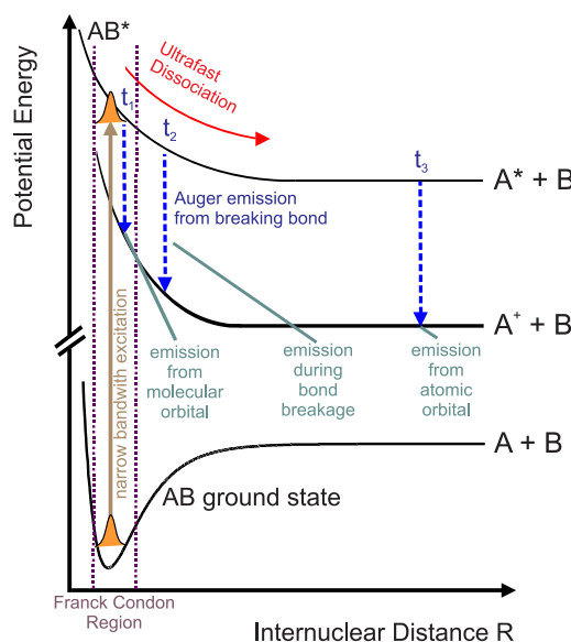
FIG. 1. Sketch of single-photon-induced ultrafast dissociation. A narrow bandwidth single photon excites an electron from an inner shell to an antibonding orbital with a steeply repulsive potential energy curve. Following this pump step, the molecule starts to dissociate. During this dissociation, the Auger electron is emitted, and the internuclear distance at the instance of decay is encoded in the electron energy and the kinetic energy of the fragments. We measure the angular distribution of this electron in the body-fixed molecular frame for different emission times or internuclear distances.
