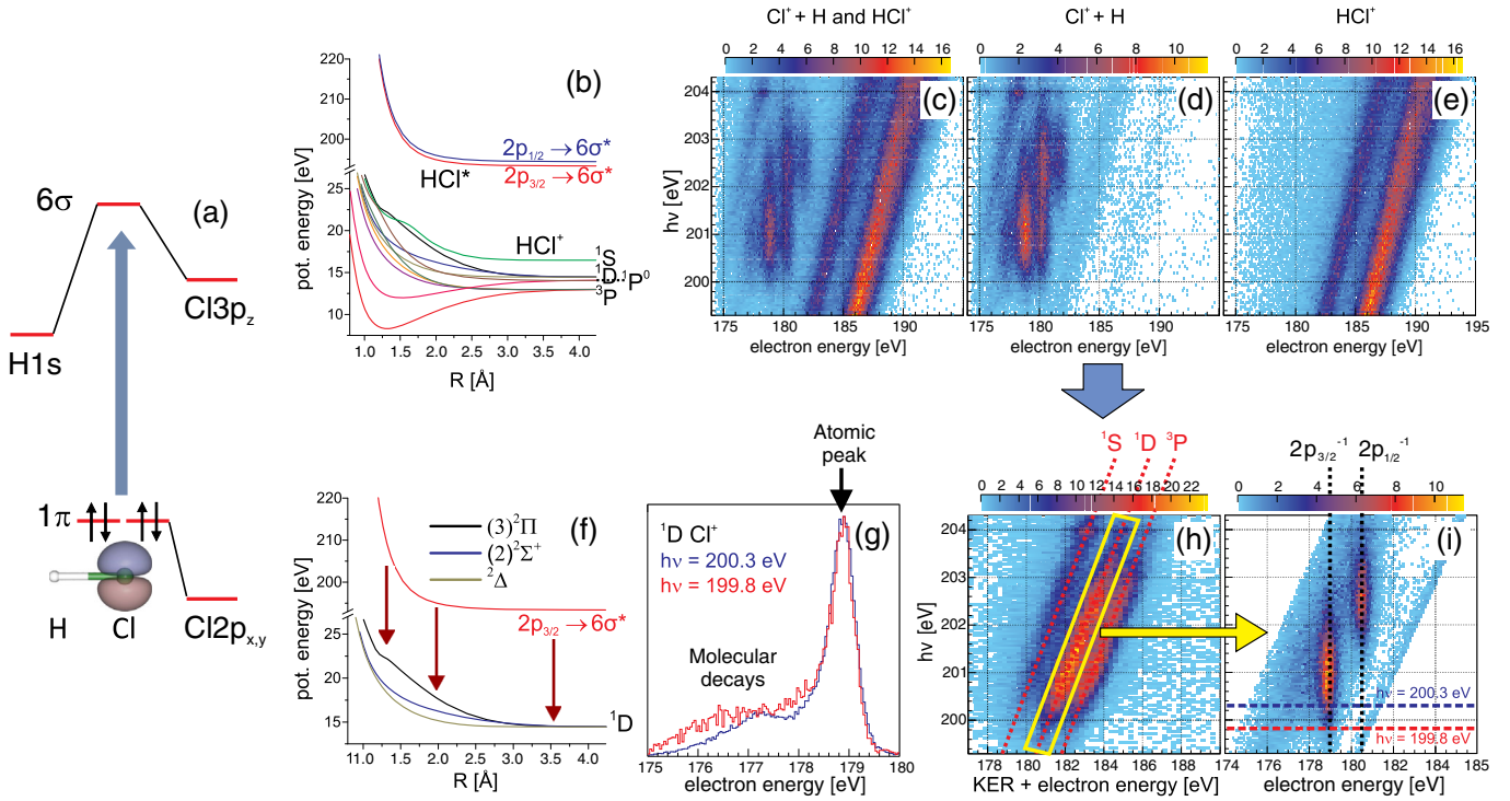
FIG. 2. Ultrafast dissociation of HCl. (a) A 1\pi electron is excited to the empty 6\sigma molecular orbital. (b) The corresponding potential energy curves [33,34]. (c) Measured electron energy distributions as a function of the photon energy without a restriction to a certain ionic channel. (d) Subset of data shown in (c) in which a coincident detection of a \text{Cl}^+ ion was required. (e) Subset of data shown in (c) which was detected in coincidence with a \text{HCl}^+ molecular ion. (f) Subset of potential energy curves depicted in (b), which is relevant for Fig. 3 and panel (g) of this figure. (g) Electron energy distributions for h\nu = 199.8 eV and h\nu = 200.3 eV and the conditions in panel (i). (h) Sum of the kinetic energy release of \text{H} + \text{Cl}^+ and electron energy versus photon energy. (i) Subset of data in (d) gated on the yellow rectangular area in panel (h).
