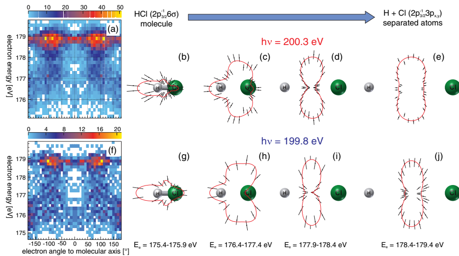
FIG. 3. (a) Electron angular emission distribution with respect to the molecular axis as a function of the electron energy obtained for the decay pathway depicted in Fig. 2(f) recorded at a fixed photon energy of h\nu = 200.3 eV. An emission angle of zero corresponds to an emission towards the \text{Cl}^+ ion. (b)–(e) Subsets of the data shown in (a) for different regions of electron energy as stated in the figures. The different polar plots correspond to steps in the decay time, i.e., a decay at a time when the molecule is still intact (b) and decays when it has already dissociated [(c),(d)] and the decay occurs in the emitted \text{Cl}^* fragment (e). (f)–(j) The same spectra as in (a)–(e) recorded at a fixed photon energy of h\nu = 199.8 eV.
