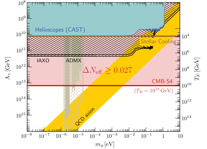
FIG. 2. Comparison between current constraints on the axion-photon coupling and the sensitivity of a future CMB-S4 mission (figure adapted from Ref. [34]). Future laboratory constraints (IA XO and ADMX) are shown as shaded regions. The yellow band indicates a range of representative models for the QCD axion. The future CMB bound is a function of the reheating temperature T_R . We note that ADMX assumes that the axion is all of the dark matter, while all other constraints do not have this restriction.
