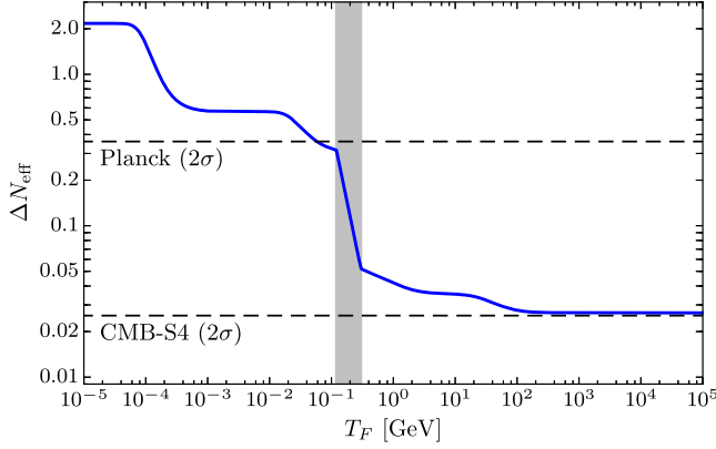
FIG. 1. Contribution of a single thermally decoupled Goldstone boson to the effective number of neutrinos, \Delta N_{\text{eff}} , as a function of the freeze-out temperature T_F . Shown are also the current 2\sigma sensitivity of the Planck satellite [1] and an (optimistic) estimate of the sensitivity of a future CMB-S4 mission [3]. The gray band indicates the QCD phase transition.
