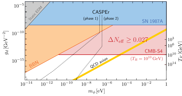
FIG. 3. Comparison between current constraints on the axion-gluon coupling and the sensitivity of a future CMB-S4 mission (figure adapted from Refs. [39,41]). The dotted lines are the projected sensitivities of the NMR experiment CASPER [42]. We note that CASPER, the static EDM [39], and BBN constraints [41] assume that the axion is all of the dark matter, while SN 1987A [15] and the future CMB constraint do not have this restriction.
