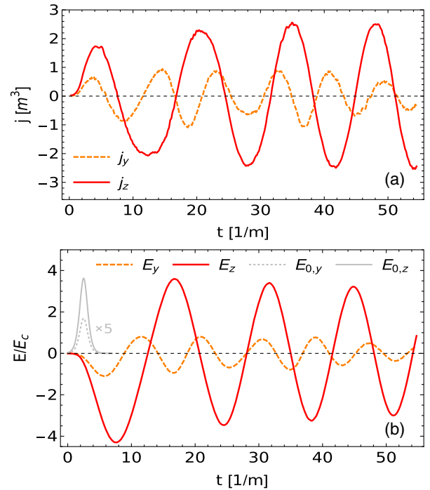
FIG. 2. Time evolution of the nonvanishing electric current and electric field components. (a) The total current results from a regular and an anomalous contribution. Accordingly, the y and z components oscillate out of phase. (b) The y and z components of the electric field are also out of phase. As a consequence, \mathbf{E} rotates relative to \mathbf{B} , cf. Fig. 3. Shown is also the initial pulse whose amplitude is rescaled by a factor of 5 for better visualization.
