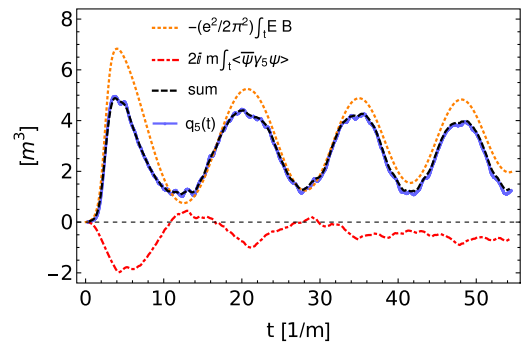
FIG. 4. Generation of the axial charge density q_5 as a function of time. In addition, the different contributions on the rhs of the space-time integrated anomaly equation (5) are shown. The fact that they sum up to give q_5 within numerical errors is a direct consequence of the quantum anomaly and an important verification of our nonequilibrium approach.
