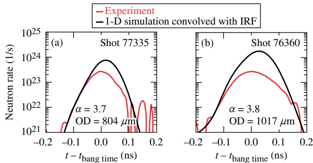
FIG. 4. Measured and 1D simulated neutron rates for \alpha = 3.7 –3.8 implosions having an initial target outside diameter (OD) of (a) 804 \mu\text{m} and (b) 1017 \mu\text{m} .
