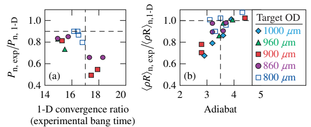
FIG. 5. (a) The ratio of measured P_{\text{hs}} to 1D simulated P_{\text{hs}} averaged over the measured neutron rate ( P_{n,\text{exp}}/P_{n,1D} ) versus the 1D simulated convergence ratio calculated at the experimental neutron bang time and (b) the ratio of measured \rho R to 1D \rho R averaged over the measured neutron rate ( \langle \rho R \rangle_{n,\text{exp}}/\langle \rho R \rangle_{n,1D} ) for targets having target outside diameters (ODs) ranging from 800 to 1000 \mu\text{m} versus the calculated shell adiabat.
