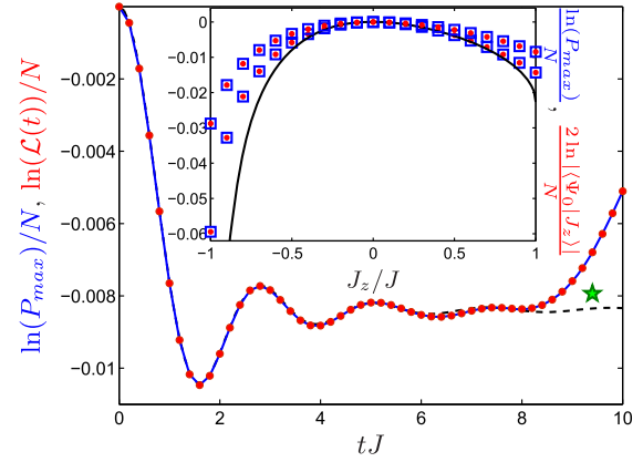
FIG. 1. The time evolution of P_{\max} , Eq. (5), (blue line) after a quantum quench for the representative case of J_z = J/2 and N = 26 is plotted, together with the overlap of the J_z = 0 and the quenched J_z = J/2 wave function (red circles), falling on top of each other (up to numerical accuracy). The upturn around tJ = 9 is due to finite size effects, following from the comparison of the infinite system result [32] (black dashed line). The green star denotes the prediction of Eq. (8), which is valid for times much larger than the transient time. The inset visualizes adiabatic results for P_{\max} (blue squares) and the overlap of the ground state wave functions (red dots) for N = 14 (upper data set) and 22 (lower data set). The ED data approach Eq. (6) (black line), which is valid in the TDL, upon increasing the system size.
