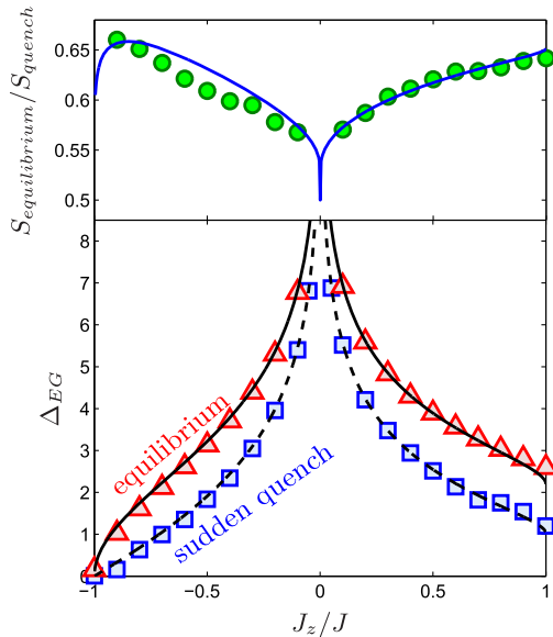
FIG. 3. Lower panel: The EG extrapolated to the TDL in equilibrium (red triangles) and after a quench (blue squares). The black solid and dashed lines depict the analytical results without any fitting parameter from Eqs. (7) and (9), respectively. Upper panel: The ratio (circles) of the von Neumann entanglement entropies in the steady state after the quench and in equilibrium from ED, extrapolated to the TDL, compared to the Luttinger model result (solid line) from Eq. (11), without any fitting.
