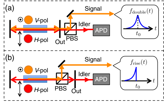
FIG. 1. Single-photon generation methods with (a) a conventional doubly resonant OPO and (b) our asymmetric OPO. Out, outcoupling mirror; APD, avalanche photodiode for idler-photon detection.
