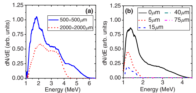
FIG. 5. (a) Measured ion energy spectra from 500 \times 500 \mu\text{m} (blue solid) and 2000 \times 2000 \mu\text{m} (red dashed) mass-limited Cu targets. (b) Ion energy spectra from the metal-PE targets with different PE thickness. The maximum energy of ions from the 40 and 75 \mu\text{m} thick PE layer becomes less than the lower detection limit (1 MeV), which is caused by the shielding Al filters in front of IP.
