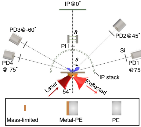
FIG. 1. Schematic of the top view of the experimental setup. The THz collection lens and windows are not shown. The lower inset sketches the three types of targets used. Pyroelectric detector (PD), pinhole (PH).
