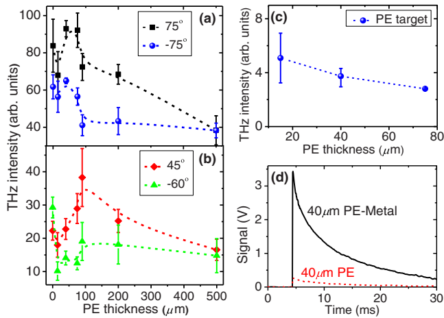
FIG. 4. (a)–(b) Measured THz intensity at 75° (black square), 45° (red diamond), -60^\circ (green triangle), and -75^\circ (blue circle) from the metal-PE targets as a function of the thickness of the PE layer. (c) Measured THz intensity at -75^\circ from the single-layer PE targets with different thickness. (d) Comparison of the typical signals recorded by the THz detector from the single-layer PE (red dashed) and the PE-metal (black solid) targets with a 40 \mu\text{m} PE layer.
