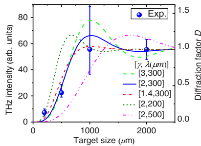
FIG. 3. Measured THz radiation intensity at -75^\circ (blue circle) and calculated diffraction modification factor D for mass-limited targets with different sizes. The solid and dashed curves are obtained with different parameters ( \gamma , \lambda ), where \gamma is the relativistic Lorentz factor of electrons and \lambda the radiation wavelength in \mu\text{m} .
