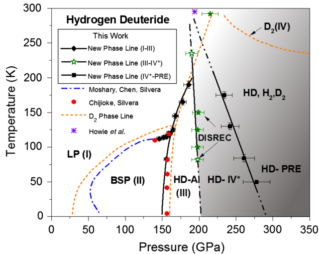
FIG. 1. The phase diagram of HD, extending the earlier measurements beyond the triple point to establish the I–III line. For comparison, we show the phase diagram of D_2 . Solid lines (above \sim 200 GPa) indicate new phase lines of mixtures of isotopes. For the III to HD-IV* line, we only traversed the phase line at P \sim 198 GPa, T = 82 , and 240 K, indicated by open stars, while DISREC was observed all along the phase line (filled stars). The shaded area shows where hydrogen, deuterium, and hydrogen deuteride spectra were observed. We also show a DISREC point at room temperature and a point from Howie et al. [12] where they observed a phase transition.
