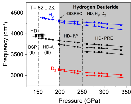
FIG. 3. Peak frequencies of the IR modes as a function of pressure, indicating phase transitions where splittings or new modes appear. The shaded area is where a mixed isotope sample, due to DISREC, was observed.
