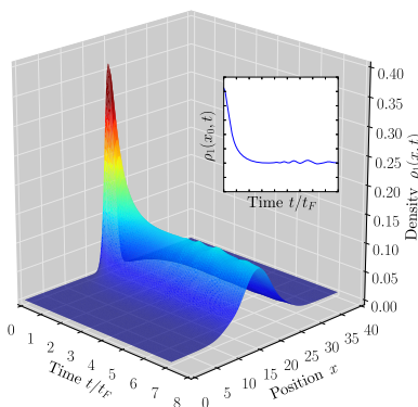
FIG. 1. Time evolution of the impurity density of the initial state (4) with Q = 0 , x_0 = L/2 , and a_0^2 = 1.125 on the L = 40 ring for a system of N = 8 particles with interaction parameter c = 10 . The Hilbert space is truncated to 25 150 states, leading to the sum rule (6) equaling 0.9858. Inset: Time evolution of the maximum of the density \rho_1(x_0, t) . Constant time cuts can be found in the Supplemental Material [61].
