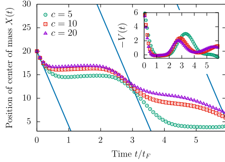
FIG. 3. The time evolution of the center of mass X(t) [Eq. (8)] for the initial state (4) with a_0^2 = 1.125 , Q = \pi for N = 8 particles on the length L = 40 ring with interaction parameter c = 5, 10, 20 (points), and a noninteracting point particle with mass m = 1/2 and velocity Q/m (line). Inset: velocity of the center of mass V(t) = \Delta X(t)/\Delta t (cf. Ref. [39]).
