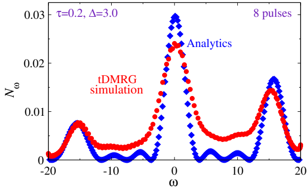
FIG. 3. Emission profiles N_\omega in the presence of control pulses, for \tau = 0.2 and \Delta = 3.0 , after the eighth pulse. Blue diamonds represent the analytical results, while the red circles represent the spectrum obtained via time-dependent density matrix renormalization group (tDMRG) simulations. The latter is rescaled by a factor 2/\pi in order to take into account different density of the photon modes between the analytical model and the 1D chain used in tDMRG simulations.
