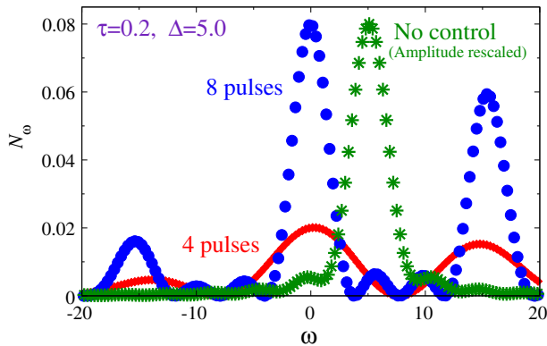
FIG. 2. Emission profile N_\omega in the presence of control pulses, for \tau = 0.2 and \Delta = 5.0 , after 4 pulses (red diamonds) and 8 pulses (blue circles), as compared with the free spontaneous emission spectrum (green stars). Amplitude of the latter is rescaled for easier comparison with the 8-pulse spectrum.
