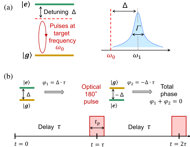
FIG. 1. (a) Excited state of the two-level system (solid-state emitter) is shifted by random amount \Delta from the desired position \omega_0 , so that the spontaneous emission line (of width \Gamma ) is centered at \omega_1 = \omega_0 + \Delta . To shift the line to the target frequency, a sequence of pulses with the carrier frequency \omega_0 is applied. (b) The optical 180^\circ control pulses are applied periodically, with the interval \tau . In the rotating frame, each pulse swaps the ground and the excited state, reversing the detuning \Delta \rightarrow -\Delta . The total phase accumulated before and after the pulse is nullified, and emission happens as if the detuning was absent, with ZPL centered at \omega_0 .
