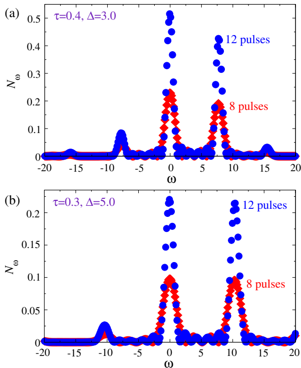
FIG. 4. Emission profiles N_\omega after 8 pulses (red diamonds) and 12 pulses (blue circles). (a) \tau = 0.4 and \Delta = 3.0 , The satellite peaks at \omega = \pm\pi/\tau and \pm 2\pi/\tau are clearly seen. (b) \tau = 0.3 and \Delta = 5.0 . Both graphs show that the protocol works for large delays \tau > 1/\Delta , delivering about 50% of emission to the target frequency.
