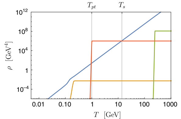
FIG. 1. The density of the vacuum energy associated with the electroweak (green line) and QCD (orange line) phase transitions, compared to the radiation energy density of the Universe (blue line), as a function of temperature. We also show the vacuum energy density associated with a new phase transition (red line), as discussed in the text. Schematically, a period of inflation occurs when the vacuum energy density exceeds the radiation energy density, starting at T_s and ending at T_{pt} . Reheating is not fully captured by this plot.
