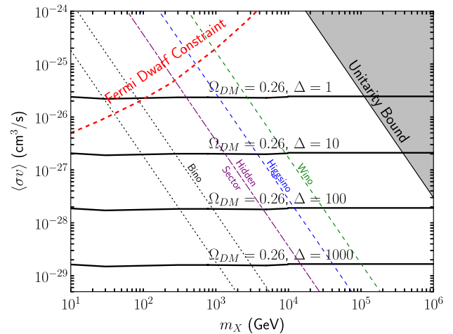
FIG. 2. The effective annihilation cross section at freeze-out for four benchmark DM models (described in the Supplemental Material [36]). The approximately horizontal thick black lines represent the values of the cross section that generate the observed dark matter density, for four different values of the dilution factor, \Delta . Large low-velocity annihilation cross sections, as shown in the upper left region, are ruled out by Fermi's observations of dwarf galaxies (assuming that the annihilation cross section is the same at low velocities and freeze-out) [48]. The upper right region is incompatible with partial wave unitarity [25].
