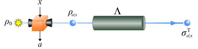
FIG. 1. Schematic diagram of temporal steering. In the beginning, Alice performs the measurement F_{a|x} = M_{a|x}^\dagger M_{a|x} on an initial state \rho_0 . Then, \rho_0 is mapped to \rho_{a|x} and sent into a quantum channel \Lambda . Finally, Bob receives the assemblage \{\sigma_{a|x}^T\} at time t .
