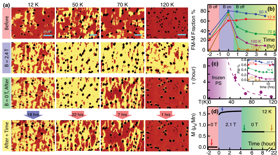
FIG. 4 (color online). (a) MIM images taken at B = 0 T (before), B = 2.4 T, B = 0 T (after), and after several hours at the same condition (after + time) at T = 12, 50, 70, and 120 K, respectively. All scale bars are 2 \mu\text{m} . (b) FM-M vs time showing the fraction before, at B = 2.4 T, turning of the B field at different T . (c) Relaxation time as a function of temperature calculated from an exponential fit of FM-M vs time. (d) Magnetization as a function of time. The B field is applied at time zero and removed after 4 hours. The arrows indicate where the MIM images were taken.
