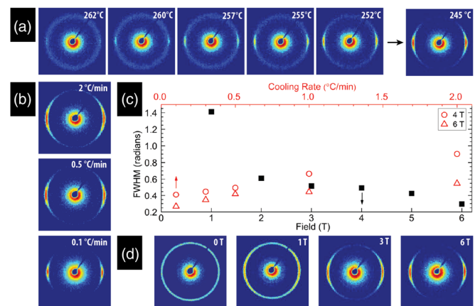
FIG. 3 (color online). (a) 2D SAXS data at selected temperatures showing the emergence of aligned lamellae during cooling from the isotropic, disordered state at 0.3 ^{\circ}\text{C}/\text{min} at 6 T. (b) Diffraction patterns for samples under 6 T at 245 ^{\circ}\text{C} after cooling across T_{\text{odt}} at the different rates indicated. (c) Dependence of azimuthal FWHM on field strength (at 0.3 ^{\circ}\text{C}/\text{min} ) and cooling rate (at 4 and 6 T), on the bottom and top x axis, respectively. (d) Diffraction patterns at 245 ^{\circ}\text{C} after cooling across T_{\text{odt}} at 0.3 ^{\circ}\text{C}/\text{min} at the indicated field strengths.
