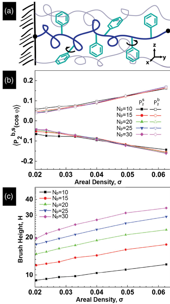
FIG. 4 (color online). (a) Illustration of a polystyrene chain tethered at an impenetrable surface. The phenyl rings can rotate around the side bond to the backbone. (b) Simulated backbone \langle P_2^b \rangle and side chain \langle P_2^s \rangle orientation distribution coefficients as functions of areal density \sigma for varying N_p . (c) Simulated brush height H(\sigma) for varying N_p .
