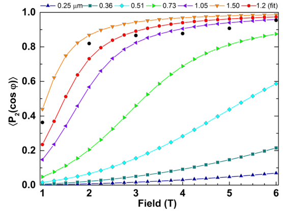
FIG. 5 (color online). Field-dependent orientation distribution coefficients [Eq. (4)] for various grain sizes \xi for \Delta\chi = -1.6 \times 10^{-8} at 245^\circ\text{C} . Black circles show experimentally derived values for samples cooled 0.3^\circ\text{C}/\text{min} . Fitting Eq. (4) (red circle trace) to experimental data yields \xi \approx 1.2 \mu\text{m} .
