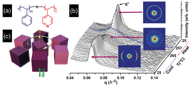
FIG. 1 (color online). (a) Chemical structure of PS-b-P4VP. (b) Temperature-resolved SAXS data ( 25 \rightarrow 265 \rightarrow 25 ^{\circ}\text{C} ) under a 6 T field applied vertically. The 2D diffractograms are shown as insets at three representative temperatures. T_{\text{odt}} = 257 ^{\circ}\text{C} , d spacing = 9.5 nm. (c) Schematic illustrating degenerate system alignment with lamellar normals perpendicular to the field.
