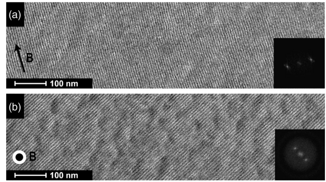
FIG. 2. TEM images and associated fast Fourier transforms (FFTs) of PS- b -P4VP aligned at 6 T, visualized (a) perpendicular to the field direction and (b) along the field direction.
