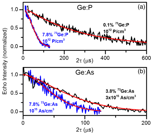
FIG. 4 (color online). Two-pulse Hahn echo decay curves for natural (blue) and isotopically enriched (black) germanium doped with phosphorus(a) and arsenic(b) donors. Data were taken at 1.8 K and 9.65 GHz. The solid curves are fits to the data using \exp[-(2\tau/T_2)^n] .
