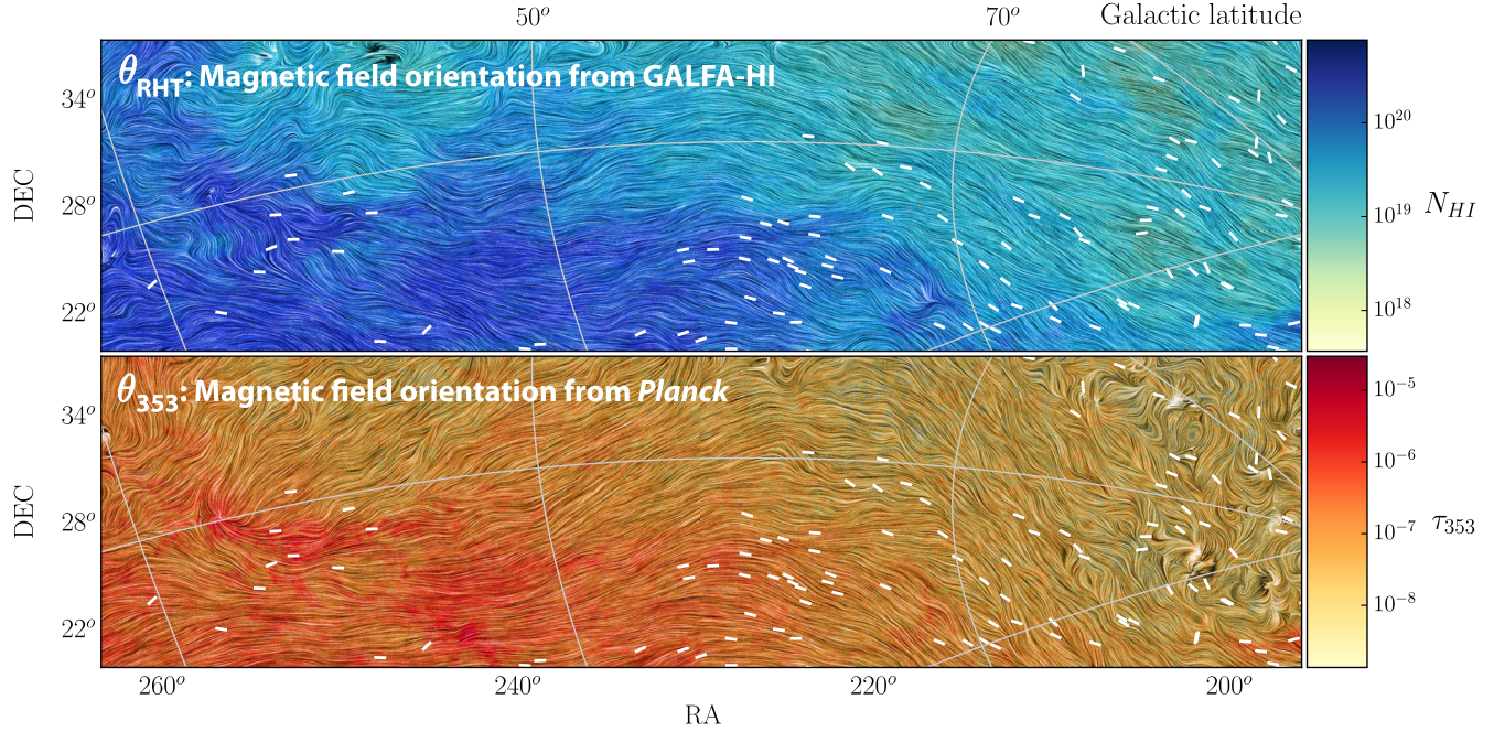
FIG. 1 (color online). Plane-of-sky magnetic field orientation as predicted by \theta_{\text{RHT}} (top) and \theta_{353} (bottom). Color maps are integrated HI column density from v = -61.5 \text{ km s}^{-1} to +61.5 \text{ km s}^{-1} ( N_{\text{HI}}[\text{cm}^{-2}] ), and dust opacity ( \tau_{353} ). Planck and RHT Q and U values are smoothed with a \text{FWHM} = 1^\circ Gaussian kernel, then used to construct \theta_{353} and \theta_{\text{RHT}} , which are visualized using line integral convolution (LIC; [24]). The high latitude ( b \gtrsim 70 ) behavior of the \theta_{353} LIC pattern is due to Planck noise. White pseudovectors represent starlight polarization angles. Galactic latitude lines lie at b = 30^\circ, 50^\circ, 70^\circ , from left to right. Galactic longitude lines lie at l = 80^\circ, 50^\circ, 20^\circ , from top to bottom.
