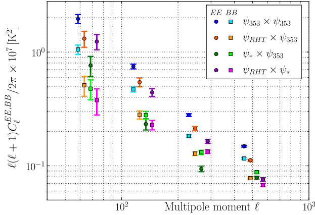
FIG. 3 (color online). Cross-power spectra of polarization template maps constructed from I_{353} and either Planck ( \psi_{353} ), RHT ( \psi_{RHT} ), or starlight polarization ( \psi_* ) data [Eq. (2)]. Shown are E -mode (circles) and B -mode (squares) components. Significant ( 40\text{--}70\sigma ) cross-correlations are detected in all cases.
