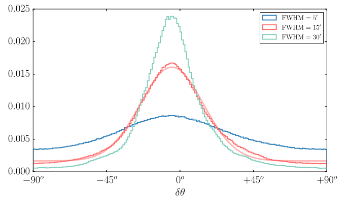
FIG. 2 (color online). Normalized histograms of \delta\theta = \theta_{353} - \theta_{\text{RHT}} in 1^\circ bins at resolutions of \text{FWHM} = 5', 15', and 30' . The Gaussian fit to the \text{FWHM} = 15' histogram shown has a standard deviation \sigma = 19.4^\circ .
