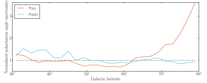
FIG. 4 (color online). Angle uncertainties averaged over 2^\circ Galactic latitude bins, normalized by their respective median values (dashed line).
