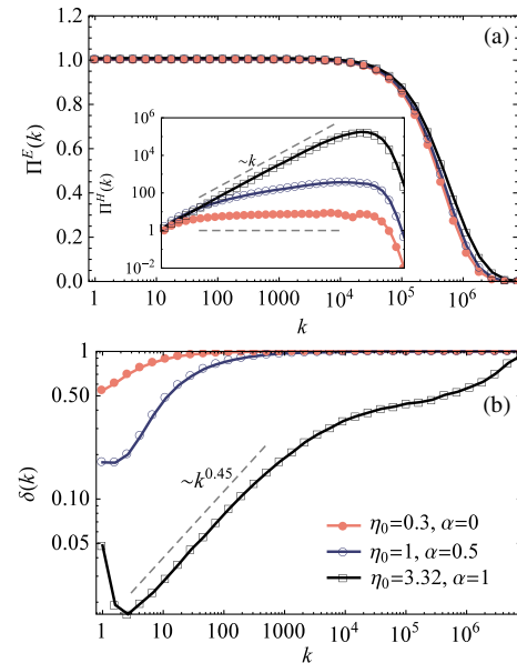
FIG. 2 (color online). (a) Spectral fluxes of energy and helicity (inset). (b) Distributions of \delta(k) = 1 - |H_r(k)| .
