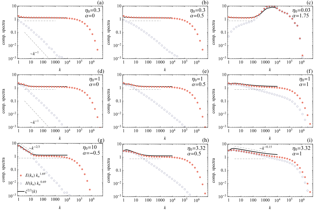
FIG. 1 (color online). Energy [E(k) , points] and normalized helicity [H(k)/k , circles] spectra compensated by k^{-1.69} (Kolmogorov's slope with intermittency correction) are shown in a grid of panels for each pairs of parameters \eta_0 = 0.3, 1, 3.32 (from top to bottom) and \alpha = 0, 0.5, 1 (from left to right). Exceptional cases are panel (c) \eta_0 = 0.03, \alpha = 1.75 and panel (g) \eta_0 = 10, \alpha = -0.5 . Theoretically predicted helical correction to the energy spectrum \zeta(k) [defined by Eq. (7)] is shown by the solid line.
