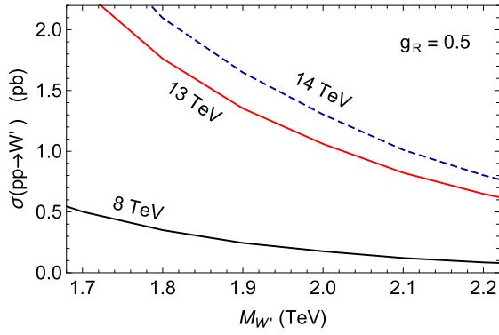
FIG. 1 (color online). Next-to-leading order cross sections for W' production at \sqrt{s} = 8, 13, and 14 TeV, for g_R = 0.5 . The cross sections scale as g_R^2 .
