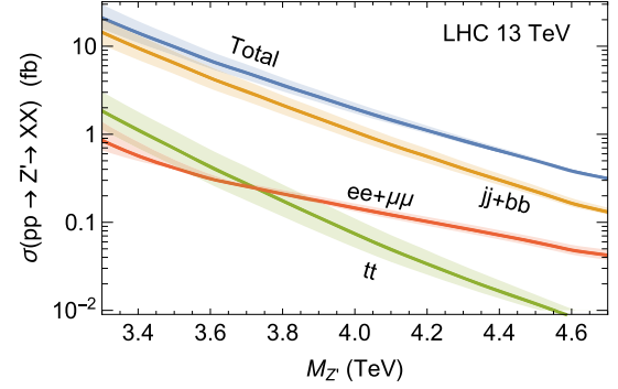
FIG. 2 (color online). Z' production cross section times branching fractions as a function of M_{Z'} , for M_{W'} = 1.9 TeV at the 13 TeV LHC. Shaded bands correspond to M_{W'} in the 1.8–2.0 TeV range.
