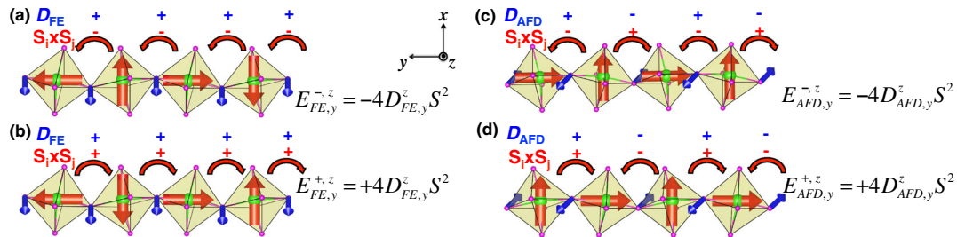
FIG. 2 (color online). Separation of FE ( \mathbf{D}_{\text{FE},k} ) and AFD ( \mathbf{D}_{\text{AFD},k} ) DM interactions in BiFeO 3 . Spin directions (red arrows) and DM vectors (blue arrows) are indicated. (a) and (b) have clockwise and counterclockwise rotation, respectively, of spins and use an 80 atom unit cell (four spins in the unit cell along each direction). (c) and (d) have zigzag-type spin ordering. \pm above red arrows denote signs of DM interaction and of spin current between two nearest-neighbor spins.
