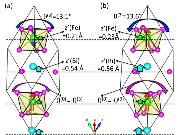
FIG. 1 (color online). First-principles relaxation results for magnetic orderings (a) G -AFM \rightarrow P = 93 \mu\text{C/cm}^2 and (b) FM \rightarrow P = 99 \mu\text{C/cm}^2 to calculate ESPs from FE distortion of Fe [ \mathbf{z}'(\text{Fe}) ] and of Bi [ \mathbf{z}'(\text{Bi}) ] along [111] and AFD R_4^+ rotations ( \theta ) perpendicular to [111] . (0) and (3) are indices of hexagonal layers ( x + y + z = n ).
