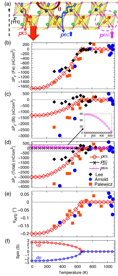
FIG. 3 (color online). (a) SD polarizations along \mathbf{z}' and AFD rotations perpendicular to \mathbf{z}' . (b) Calculated Fe polarizations along \mathbf{z}' induced by ES ( P^{ES} ) compared with measurements by Lee et al. [6], Arnold et al. [8], and Palewicz et al. [12]. (c) Bi polarizations along \mathbf{z}' induced by ES. (d) Total SD polarization \Delta P_{z'}(\text{Fe}) + \Delta P_{z'}(\text{Bi}) . The inset is the SC polarization calculated from Eqs. (21) and (22) and Ref. [25]. (e) Change of AFD-rotation angle induced by ES. (f) AFM spin ordering versus temperature calculated by mean-field theory.
