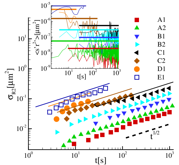
FIG. 1 (color online). Root mean square of the square droplet radius fluctuations \sigma_{R^2} versus time from simulations (symbols) and the prediction of the stochastic model (13) (lines). Inset: correlation \langle s'R^2 \rangle from simulations (thin lines) and from Eq. (12) (thick lines).
