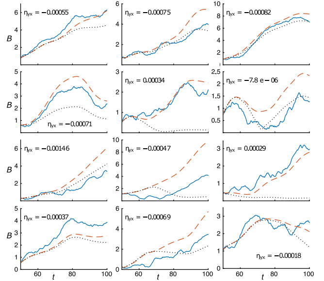
FIG. 4 (color online). Evolution of the mean-field magnitude for a sample of the ensemble of rotating simulations (Figs. 2 and 3). Here B , the mean-field magnitude, is (|\hat{B}_x^1|^2 + |\hat{B}_y^1|^2)^{1/2} , where \hat{B}_i^1 is the largest scale Fourier mode of B_i . In each plot the solid blue curve shows data taken from the simulation. The dashed red curve shows the corresponding expected evolution, using the time-dependent calculated values of the transport coefficients, smoothed in time using a Gaussian filter of width 5. Finally, the dotted black curve illustrates the expected evolution with all \alpha coefficients artificially set to zero. The similarity between this evolution and that including \alpha (dashed curve) illustrates that in many (but not all) cases the dynamo is primarily driven by \eta_{yx} . We list the measured mean of \eta_{yx} in each plot to show that lower values generally lead to stronger mean-field growth, as expected for a coherent dynamo. For reference, at the measured \eta_{xx} \approx 0.006 , the coherent dynamo is unstable below \eta_{yx} = -0.00036 .
