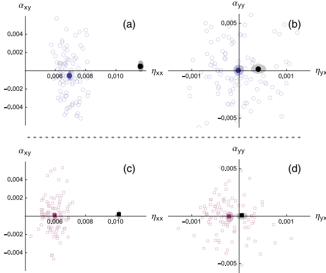
FIG. 3 (color online). Measurements of the turbulent transport coefficients for 100 realizations of the simulations at the same parameters as those in Fig. 2; (a) \eta_{xx} and \alpha_{xy} coefficients ( x and y axes, respectively), no rotation, (b) \eta_{yx} and \alpha_{yy} coefficients, no rotation, (c) \eta_{xx} and \alpha_{xy} coefficients, rotating, (d) \eta_{yx} and \alpha_{yy} coefficients, rotating [see Eq. (3)]. Unfilled markers in each plot show coefficients measured from each of the individual realizations, with mean values displayed with solid markers and the shaded regions indicating error in the mean (2 standard deviations). Black markers illustrate the kinematic transport coefficients, with grey shaded regions indicating the error. After saturation of the small-scale dynamo, we calculate \alpha_{ij}(t) and \eta_{ij}(t) by solving Eq. (2) approximately (see text), taking the mean from t = 50 to t = 100 . This limited time window is chosen to avoid capturing the saturation phase of the large-scale dynamo, since \eta_{ij} is presumably modified in this phase. In both methods of computing transport coefficients, \alpha coefficients are zero to within error as expected, and the scatter between simulations is of a similar magnitude to that of \eta_{ij} if one accounts for their different units (it is necessary to divide \alpha by a characteristic k value).
