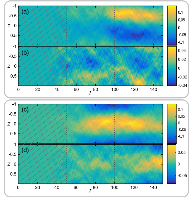
FIG. 2 (color online). Example spatiotemporal B_y evolutions for nonrotating [(a), (b)] and Keplerian rotating [(c), (d)] turbulence at Re_m = u_{rms}/\eta k_f \approx 15 ( k_f = 6\pi , \eta = 1/2000 , Pm = 8 , S = 1 , in a box of dimension (1, 4, 2) with resolution (64, 128, 128) . The first examples in each case [(a) and (c)] show B_y when a coherent dynamo develops, while the second examples [(b) and (d)] illustrate the case when it is more incoherent. The main factors in distinguishing these are the coherency in phase of B_y over some time period and the amplitude at saturation, which is larger in the coherent cases. In general, the rotating simulations are substantially more coherent. The hatched area illustrates the region of small-scale dynamo growth. The fitting method used to compute transport coefficients (see Fig. 3) is applied between the dashed lines ( t = 50 \rightarrow 100 ).
