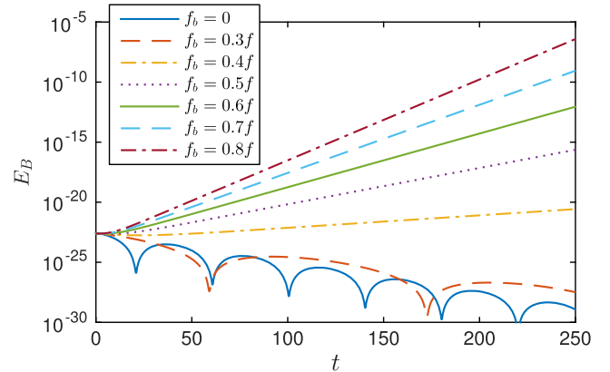
FIG. 1 (color online). Time development of the mean-field energy, E_B = \int dz B^2/2 , in quasilinear statistical simulation. Small-scale fields are forced at k_f = 6\pi , \text{Re}_m = u_{\text{rms}}/\eta k_f \approx 5 (here \eta is the resistivity, \text{Pm} = \text{Re}_m/\text{Re} = 1 ), S = 2 and the box has dimensions (L_x, L_y, L_z) = (1, 1, 4) with resolution (28, 28, 128) . As well as forcing the momentum equation, the induction equation is forced to excite homogeneous magnetic fluctuations, emulating a small-scale dynamo. Total forcing is kept constant in each simulation but the proportion of magnetic forcing ( f_b/f ) is increased from 0 to 0.8 [28]. As f_b/f increases, the growth rate of the mean field increases due to the change in sign and subsequent decrease of \eta_{yx} .
