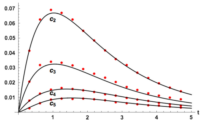
FIG. 2 (color online). Theoretical and simulated cluster densities c_2(t) through c_5(t) . Solid lines show theoretical predictions computed from numerical integration of Eq. (6). Data points show simulation results for N = 5 \times 10^4 oscillators.
