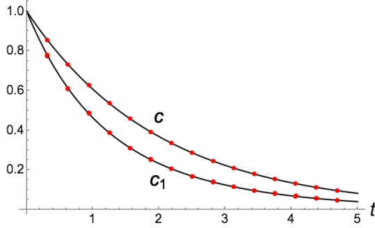
FIG. 1 (color online). Theoretical and simulated c(t) and c_1(t) . Solid lines show theoretical curves obtained analytically (see text). Data points show simulation results for N = 10^4 oscillators.
