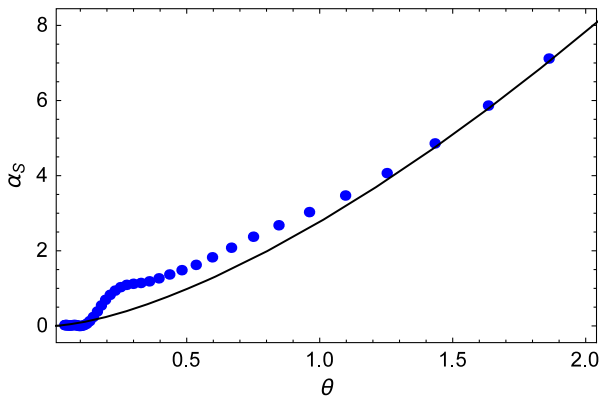
FIG. 2 (color online). Local shear viscosity coefficient \alpha_S (blue dots) versus reduced temperature \theta = T/T_F(n) . The prediction from the two-body Boltzmann equation [12] 2.77\theta^{3/2} (black curve) is used as a seed function to initialize the iteration procedure and as a constraint at large \theta .
