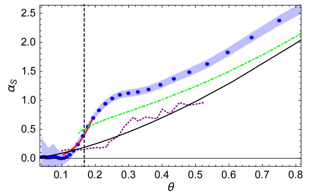
FIG. 3 (color online). Extracted local shear viscosity coefficient \alpha_S (blue dots) versus reduced temperature \theta = T/T_F(n) near the superfluid transition temperature, where the local shear viscosity is \eta = \alpha_S(\theta)\hbar n . The vertical dashed line denotes the critical temperature \theta_c = 0.167(13) [18]. Blue bands denote the standard error corresponding to the statistical uncertainty in \langle \alpha_S \rangle ; Red solid line from Guo et al. , Ref. [4]; Green dotted curve from Enss et al. , Ref. [15]; Purple dot-dashed curve from Wlazlowski et al. , Ref. [16]; Black-solid line prediction from kinetic theory \alpha_S = 2.77\theta^{3/2} [12].
