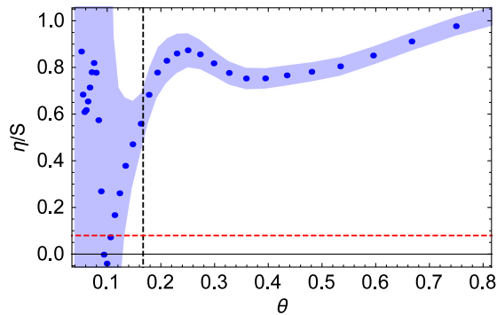
FIG. 5 (color online). Ratio of shear viscosity \eta to the entropy density s , in units of \hbar/k_B , versus reduced temperature \theta = T/T_F(n) . Blue dots are the ratio of the local shear viscosity, obtained from our matrix inversion method, to the entropy density measured in Ref. [18]. Blue bands denote the standard error for quadratically combining the statistical uncertainties in \langle \alpha_S \rangle and in s . The vertical dashed line denotes the critical reduced temperature and the horizontal dashed line at 1/(4\pi) indicates the KSS lower bound [1].
