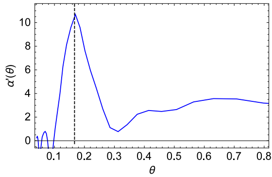
FIG. 4 (color online). Slope of the shear viscosity coefficient \alpha'_S versus reduced temperature \theta , showing a peak at T_c . The vertical dashed line denotes the critical reduced temperature.
