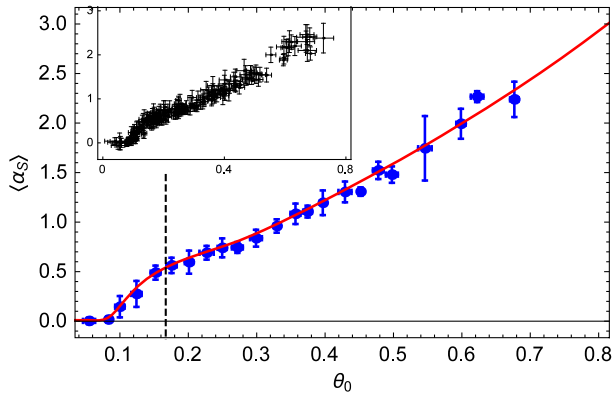
FIG. 1 (color online). Trap-averaged shear viscosity coefficient \langle\alpha_S\rangle , where the shear viscosity is \eta = \alpha_S \hbar n . The solid blue points show the \langle\alpha_S\rangle data versus reduced temperature \theta_0 at the trap center, after binning the raw data (inset) in \theta_0 . The vertical dashed line denotes the critical temperature at the trap center \theta_c = 0.167(13) [18]. The red solid line is obtained by integrating \alpha_S(\theta) , which is estimated from the \langle\alpha_S\rangle data using an image processing algorithm.
