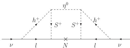
FIG. 3. Another three-loop neutrino mass.
