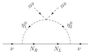
FIG. 5. One-loop U(1)_D scotogenic neutrino mass.
