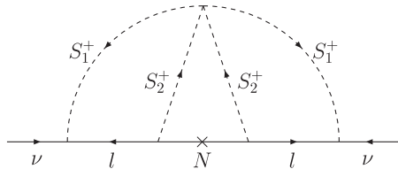
FIG. 2. Three-loop neutrino mass.
