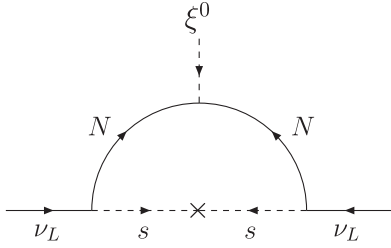
FIG. 6. One-loop neutrino mass from L = 0 Higgs triplet.
