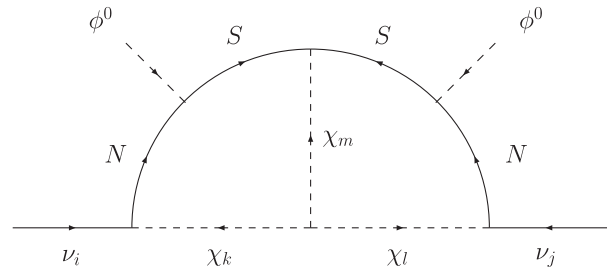
FIG. 4. Two-loop neutrino mass.
