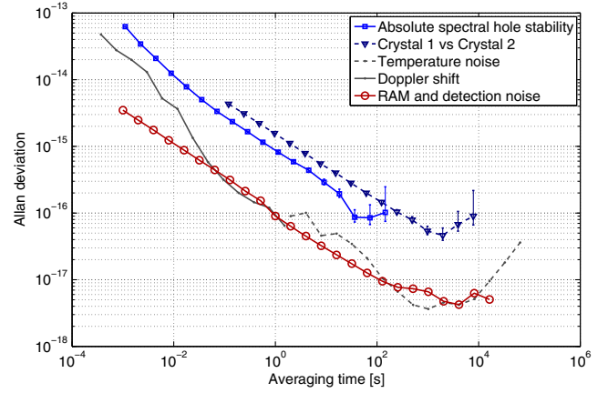
FIG. 8 (color online). Fractional frequency instability of a laser locked to a steady-state pattern of spectral holes in \text{Eu}^{3+}:\text{Y}_2\text{SiO}_5 . Absolute laser-frequency instability from a three-cornered hat measurement is shown (blue squares), as well as the differential instability of a crystal versus crystal frequency comparison (triangles) where much of the technical noise is common mode. The instability of the crystal versus crystal measurement is worse at small averaging times because the duty cycle is 50%, while the absolute spectral-hole stability measurement uses feedback from both crystals to achieve 100% duty cycle. The expected frequency noise due to temperature fluctuations (dashed gray line), Doppler shifts due to motion of the pillbox (solid gray line), as well as RAM and detection noise (open red circles) are also shown.
