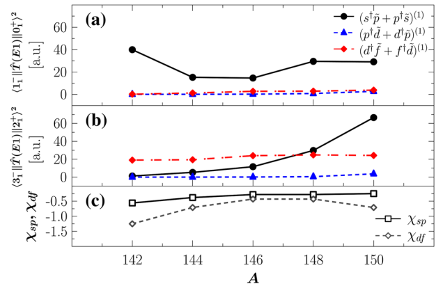
FIG. 3 (color online). E1 matrix element (a) \langle 1^- | \hat{T}(E1) | 0_1^+ \rangle^2 and (b) \langle 3^- | \hat{T}(E1) | 2_1^+ \rangle^2 for ^{142-150}\text{Nd} . Shown are the bare contributions to the spdf IBM E1 operator of Eq. (2). No fit parameters have been adjusted. (c) Evolution of the fit parameters \chi_{sp} and \chi_{df} in Eq. (2) used to describe the experimental E1 strength.
