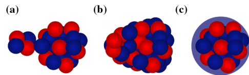
FIG. 1 (color online). Macroscopic interpretations of the different low-lying dipole modes. (a) \alpha -clustering mode, (b) octupole mode, and (c) neutron-skin oscillation [pygmy dipole resonance (PDR)].
