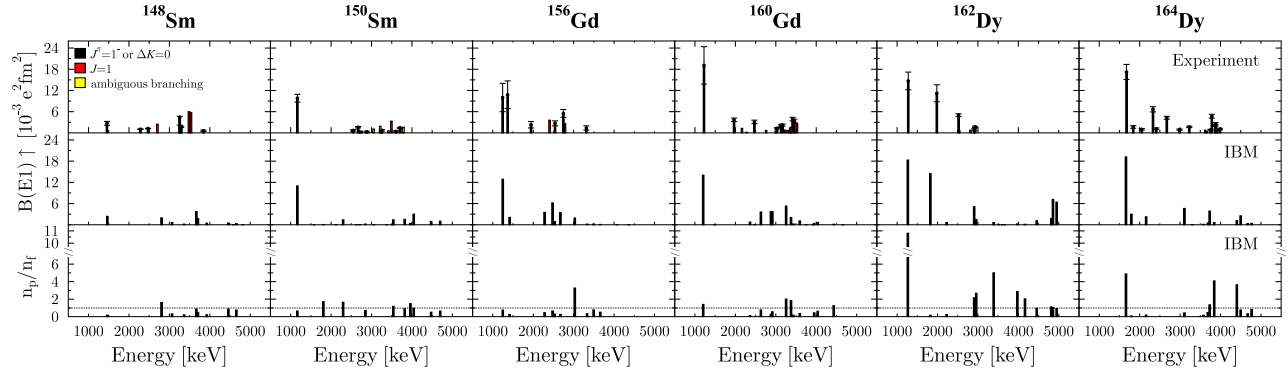
FIG. 4 (color online). Same as Fig. 2 but for ^{148,150}\text{Sm} , ^{156,160}\text{Gd} , and ^{162,164}\text{Dy} . In addition, states with an experimentally ambiguous \gamma -decay branching are marked in yellow.
