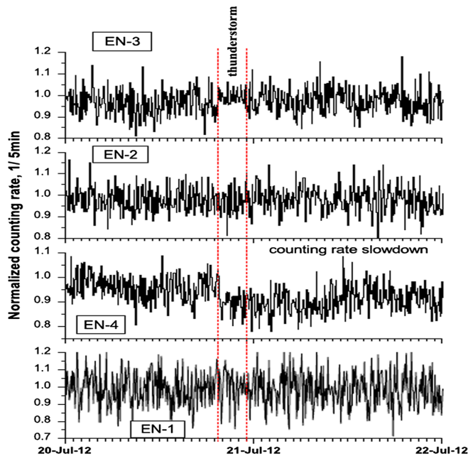
FIG. 4 (color online). Normalized neutron counting rate as a function of the time recorded by the A1 detectors installed at MEPhI-Moscow. The two vertical dashed lines define the duration of the thunderstorm that occurred on 20 July 2012. Pressure corrected data.
