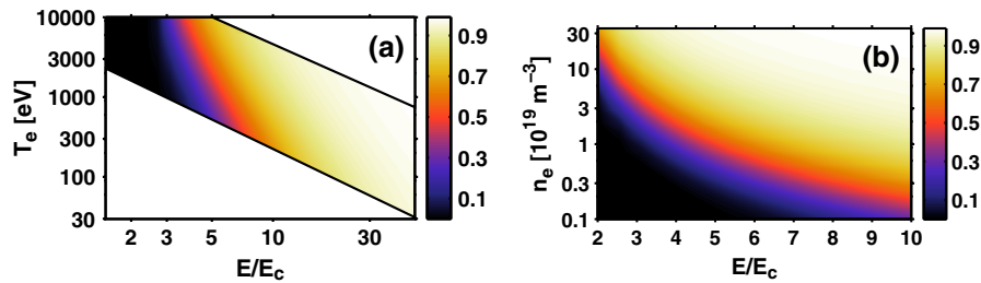
FIG. 3 (color online). Contour plots of the (a) temperature and (b) density dependence of the ratio between the primary RE growth rate in CODE with and without synchrotron effects included. The parameters B = 4 T, Z_{\text{eff}} = 1.5 , and (a) n_e = 1 \times 10^{19} \text{ m}^{-3} , (b) T_e = 2 keV were used. To ensure reliable results in (a), the parameter region has been restricted as the growth rates are negligible for low T_e and E fields, and E/E_D approaches unity for high T_e and E fields (cf. Fig. 2).
