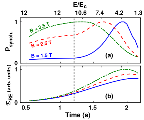
FIG. 4 (color online). (a) Emitted synchrotron power in the visual range and (b) kinetic energy contained in the RE population during electric field ramp-down. In (a), each curve is normalized to its peak value. The parameters T_e = 1.1 keV, n_e = 2.5 \times 10^{19} \text{ m}^{-3} , and Z_{\text{eff}} = 1.2 were used. The black dotted lines denote the beginning of the E -field ramp-down phase.
