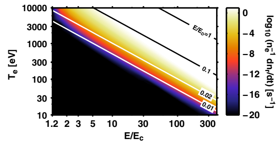
FIG. 2 (color online). Primary runaway growth rate (particle fraction per second) as a function of temperature and electric field, in the absence of synchrotron effects. White and black contours refer to E/E_D . The plasma parameters n_e = 5 \times 10^{19} \text{ m}^{-3} and Z_{\text{eff}} = 1.5 were used.
