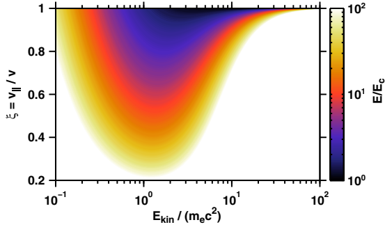
FIG. 1 (color online). Magnitude of the normalized electric field ( E/E_c ) necessary to compensate for collisional friction and synchrotron damping for a single electron in an ITER-like plasma with n_e = 10^{20} \text{ m}^{-3} , T_e = 10 \text{ keV} , and B = 5 \text{ T} .
