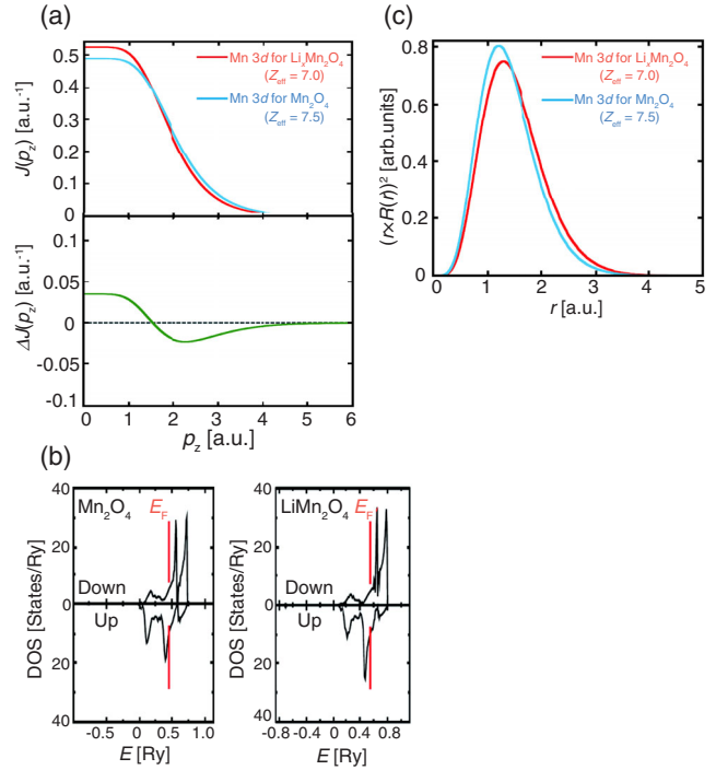
FIG. 3 (color online). Effect of Mn 3d localization on electron momentum density distribution. (a) Upper panel: hydrogenlike atomic orbital calculations simulate the effect of Mn 3d localization on electron momentum density distribution (Compton profile), where the effective charge ( Z_{\text{eff}} ) is 7 for \text{Li}_x\text{Mn}_2\text{O}_4 (red curve) and 7.5 for \text{Mn}_2\text{O}_4 (blue curve). Lower panel: the difference between \text{Li}_x\text{Mn}_2\text{O}_4 and \text{Mn}_2\text{O}_4 reproduces the negative part between p_z = 1.5 a.u. and p_z = 2 a.u. observed in experiment [Fig. 1(a)]. (b) Mn 3d partial DOS for \text{Mn}_2\text{O}_4 and \text{Li}_x\text{Mn}_2\text{O}_4 from KKR CPA calculations. The peaks of the Mn 3d partial DOS become more atomiclike as the Li concentration increases. (c) Radial wave function of the Mn 3d orbital. Insertion of Li induces a delocalization of the d electrons in real space.
