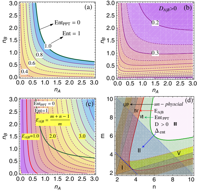
FIG. 2 (color online). Contour plots show the effect of asymmetric noises n_A and n_B on quantum correlation, for the two-mode STS with r = 0.6 : (a) entanglement measured by Ent, (b) discord measured by D_{A|B} , and (c) the steering parameter E_{A|B} . In (c), the states can be used as quantum resources with EPR steering (below red curve), entanglement (below green curve), or discord beyond entanglement (above green curve) as explained in text. (d) shows the different regions defined in Fig. 1 certified by criteria of steering, entanglement, discord, and unphysical CMs (light gray area UP) versus n and m .
