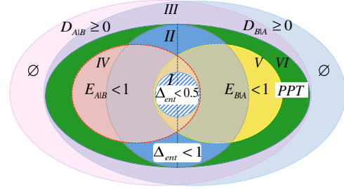
FIG. 1 (color online). The Venn diagram relations classifying the different types of quantum correlation for two-mode, two-party Gaussian states. The larger blue circle II contains states satisfying the Tan-Duan criterion for entanglement \Delta_{\text{ent}} < 1 . The inner blue circle I contains states with the symmetric two-way EPR steering correlation given by \Delta_{\text{ent}} < 0.5 . The set of all entangled states quantified by the Simon-PPT criterion \text{Ent}_{\text{PPT}} < 0 (equivalent to \text{Ent} < 1 ) are contained in the larger green ellipse VI. The smaller orange-pink IV and yellow V ellipses enclose states that display the directional steering, given by the EPR-Reid paradox condition E_{A|B} < 1 and E_{B|A} < 1 , respectively. Their intersection (colored dark yellow) is the set of two-way steerable states, which is a strict superset of the states in I. All two-way steerable states are a subset of the entangled states quantified by the Tan-Duan condition \Delta_{\text{ent}} < 1 . One-way steering states are a strict subset of the PPT entangled states, and are strictly not contained in the Tan-Duan circle \Delta_{\text{ent}} < 1 . The symmetric states with g_{\text{sym}}^{A|B} = 1 ( n = m ) are depicted at the very center of the diagram (dashed line). Those with g_{\text{sym}}^{A|B} > 1 ( n > m ) are to the right of the centre line; those with g_{\text{sym}}^{A|B} < 1 ( n < m ) to the left. The outer ellipse III contains the set of Gaussian states with nonzero quantum A and B discord.
