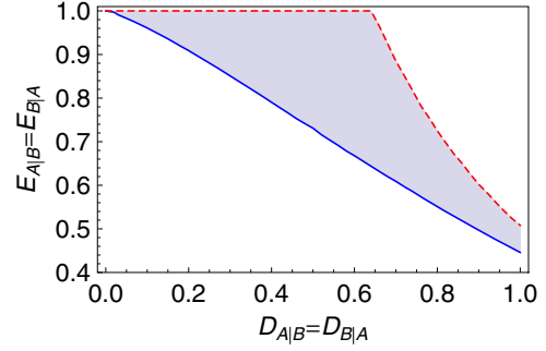
FIG. 3 (color online). The allowed Gaussian steerability (shaded region) versus discord for the symmetric Gaussian case restricting to c_1 = -c_2 = c and n = m .
