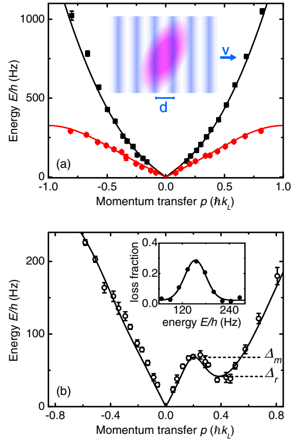
FIG. 2 (color online). Excitation spectra. (a) We measure the excitation spectra with N_0 = 30000 atoms in a harmonic trap (square) and in a stationary lattice (circle) with DMD-based Bragg spectroscopy. The inset illustrates the moving optical potential with velocity v and periodicity d created by the DMD on the BEC (tilted ellipse); see text. The solid lines correspond to the Bogoliubov model with chemical potentials equal to the trap-averaged values. (b) For a BEC with N_0 = 9000 atoms loaded in a shaken optical lattice, we measure the excitation spectrum along the lattice direction. The modulation amplitude (peak to peak) is \Delta x = 33 nm. The solid line is the best fit based on Eq. (1). The inset shows a typical atom loss spectrum taken at k = -0.38 k_L . In both panels, the scattering length is a = 47 a_0 .
