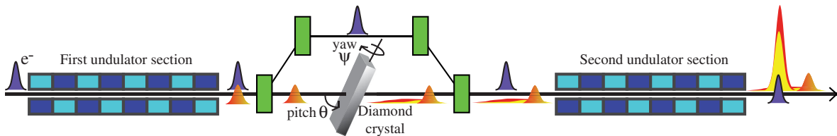
FIG. 1 (color online). Single-crystal self-seeding scheme at LCLS. In the first undulator section a self-amplified spontaneous emission (SASE) photon pulse is generated. This photon pulse diffracts from a diamond crystal. The diffracted bandwidth is at least an order of magnitude smaller than the SASE bandwidth. The diffracted beam exits at some angle to the incident beam and is discarded. The undiffracted, transmitted pulse consists of a wide-bandwidth short pulse followed by a relatively weak narrow-bandwidth tail. The electron pulse is delayed by the magnetic chicane to overlap spatially with the narrow-bandwidth tail of the x-ray pulse in the second undulator section. The narrow-bandwidth tail, with long temporal coherence length, seeds FEL amplification in the second undulator section, generating a narrow-band intense x-ray output.
