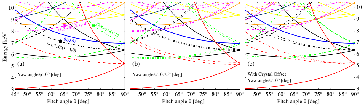
FIG. 2 (color online). Photon energy values at which diffraction occurs in a diamond crystal, as a function of the pitch angle \theta for fixed values of yaw angle \psi . Each curve corresponds to reflection from a different set of crystallographic planes. (a) Yaw angle \psi = 0^\circ . Stars represent demonstrated two-color working points. (b) Yaw angle \psi = 0.75^\circ . Different colors represent planes with different h^2 + k^2 + l^2 value. Dash-dotted lines are double lines (two sets of crystal planes excited) that are superposed for \psi = 0^\circ and can be separated with a nonzero yaw angle. (c) Correcting for the small crystal orientation offset deduced from experimental measurements of the energies as a function of (\theta, \psi) values.
