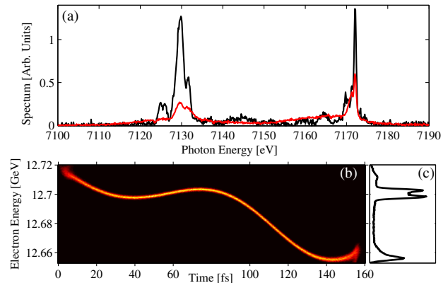
FIG. 5 (color online). (a) Two-color self-seeded spectrum obtained by using the (\bar{1}13) and (1\bar{1}3) reflections, single shot (black) and average on 100 shots (red). The two color lines are separated by 43 eV ( \sim 0.6\% ), which is wider than the SASE bandwidth for the normal LCLS operation. The pulse energy for the shot was 120 \mu J. (b) LITRACK simulated phase space obtained by manipulating the X band linearizer. (c) Simulated two energy level electron beam energy profile.
