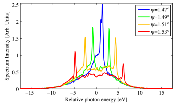
FIG. 3 (color online). Average spectra from 111 consecutive shots for single-crystal two-color self-seeded beams with photon energy close to 8.43 keV. The pitch angle was fixed to \theta = 65.28^\circ . (Blue) yaw angle \psi = 1.47^\circ . (Green) \psi = 1.49^\circ . (Orange) \psi = 1.51^\circ . (Red) \psi = 1.53^\circ . The used reflection planes were (13\bar{3}) and (31\bar{3}) . The average spectra are shown without postprocessing, including the SASE prepulse. The plateau between the two narrow colors is mainly due to the wide-bandwidth head part amplified in the second undulator section.
