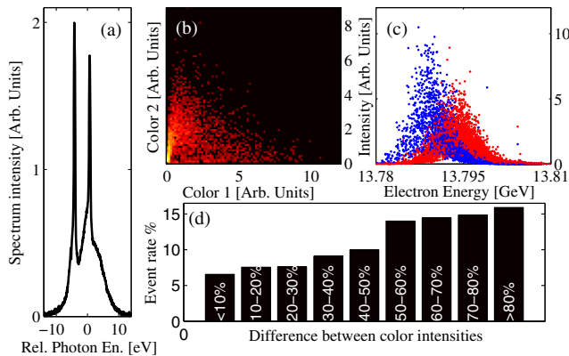
FIG. 4 (color online). Single-crystal two-color self-seeding experimental results for 3500 consecutive shots. Photon energy was close to 8.43 keV and the reflections used were (202) and (022). (a) Average spectrum. (b) Correlation between the first and second color intensities in a 1 eV bandwidth around each color average peak energy. (c) Single-shot intensities in a 1 eV bandwidth for both colors vs electron beam energy; (blue) color 1; (red) color 2. (d) Histogram of the event rate as a function of the difference between the intensities of the two colors.
