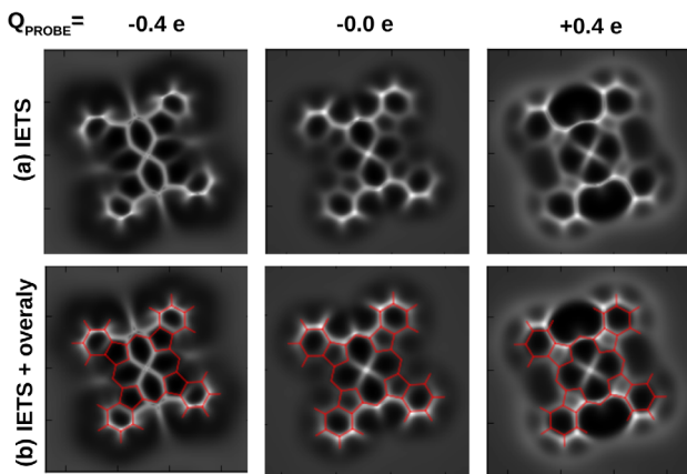
FIG. 3 (color online). Simulated constant-height IETS-STM images calculated at tip-sample distance z = 7.3 \text{ \AA} at V = 1.5 \text{ mV} for different point charge values on the probe particle, Q = -0.4e , 0 , and +0.4e . (a) IETS-STM images. (b) The same images as in panel (a), overlaid with the molecular skeleton (red line) of the relaxed CoPc molecule on Ag(110) obtained by the DFT calculations. Bright color indicates a large intensity of the IETS signal; see [29].
