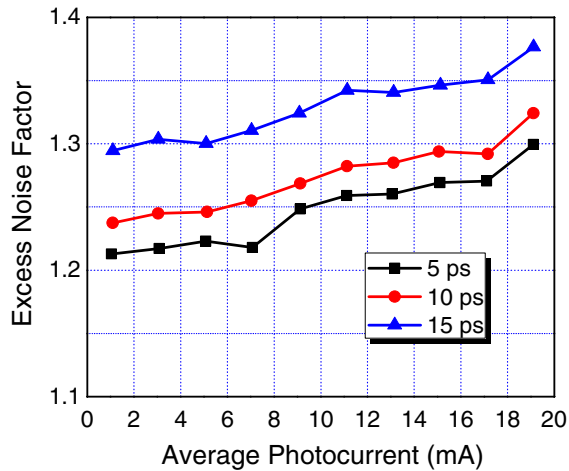
FIG. 4 (color online). Average photocurrent and optical pulse width dependence of F_H at 10 GHz.
