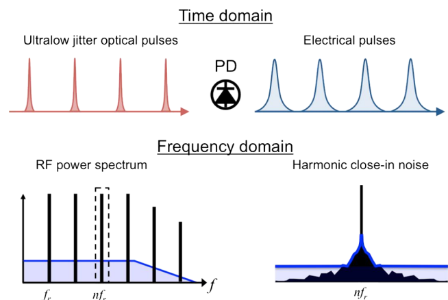
FIG. 1 (color online). Schematic diagram of photonic microwave generation via the detection of ultralow jitter optical pulses. In the lower right, the black noise sidebands represent the noise from the optical pulse train, and the blue line is the total noise after photodetection.
