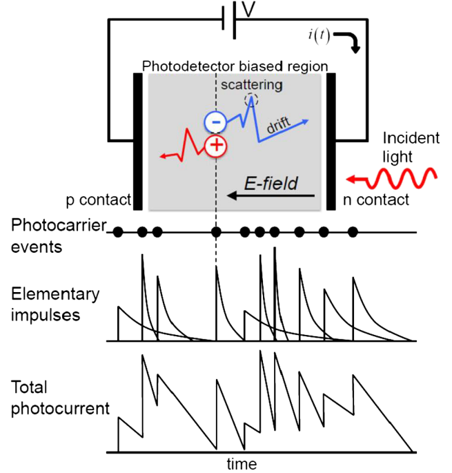
FIG. 2 (color online). Simplified schematic illustration of photocarrier transport and resulting photocurrent from a reverse-biased photodiode. Both the randomness in the timing of the photoelectron events and the shape of the elementary impulses give rise to noise in the photocurrent.
