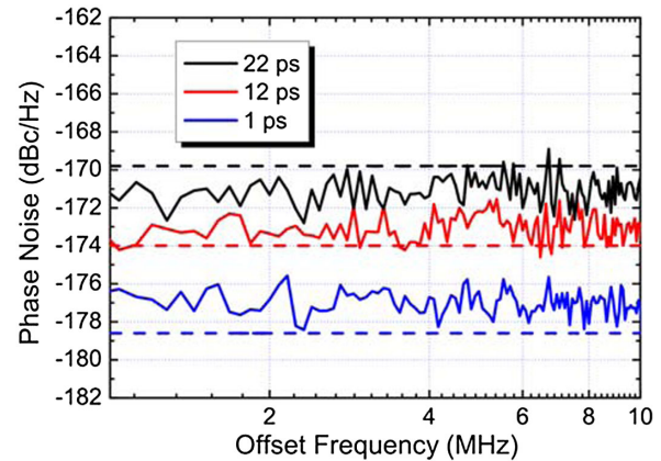
FIG. 5 (color online). Simulated single sideband phase noise level at three selected pulse widths. Dashed lines are the corresponding experimental results from Ref. [10].
