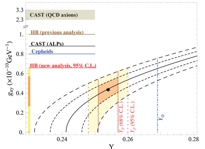
FIG. 1 (color online). R parameter constraints to Y and g_{a\gamma} . The vertical lines indicate, respectively, the 1\sigma (short-dotted curves) and 2\sigma (long-dotted curves) of Y . The dotted-dashed vertical line indicates the preferred value of Y_\odot . The other bent curves correspond to the determination of g_{a\gamma} as a function of Y from R_{\text{th}} [Eq. (1)]. Specifically, the continuous curve corresponds to R_{\text{th}} = R_{\text{av}} , while the short and long-dashed lines indicate, respectively, the 1\sigma and the 2\sigma ranges. The star represents the best fits for Y = 0.254 . The shaded area delimits the combined 68% C.L. (dark) and 95% C.L. (light) for Y and R_{\text{th}} . The vertical rectangles indicate the 68% C.L. (dark) and 95% C.L. (light) for g_{a\gamma} . Previous bounds from HB lifetime [27], from the Cepheids observation [30], from CAST for light ALPs [25,26] and for QCD axions [23] are also shown.
